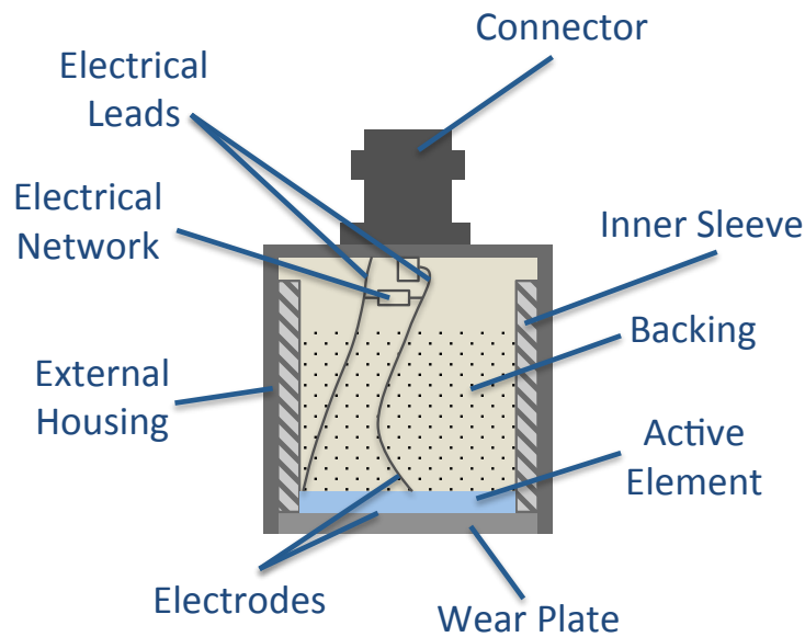
Figure 2.3: Main components of a piezoelectric transducer.
