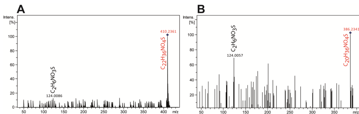
Figure 5-3 Experimental (-) TOF-MS/MS spectra: A: N-arachidonoyltaurine; B: N-linoleoyl taurine
