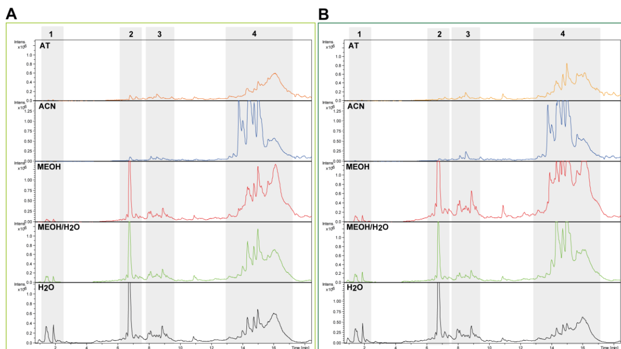
Figure 4-4 Total ion chromatograms of the solvent extraction procedure and the homogenization types derived from (-) UPCL-TOF-MS measurements
