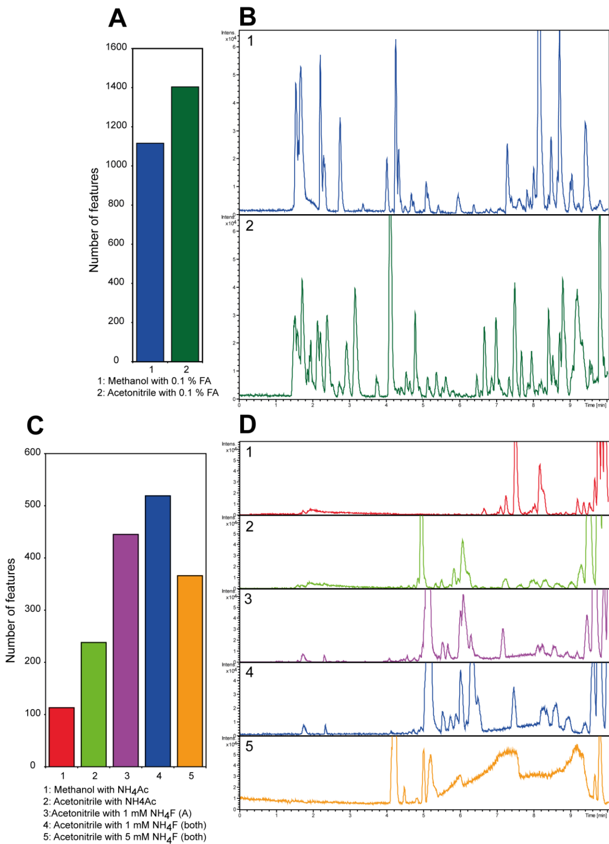
Figure 4-9 A-B: Additives evaluation in (+) UPLC-TOF-MS mode and their respective TICs; C-D: Additive evaluation in (-) UPLC-TOF-MS mode and their respective TICs
