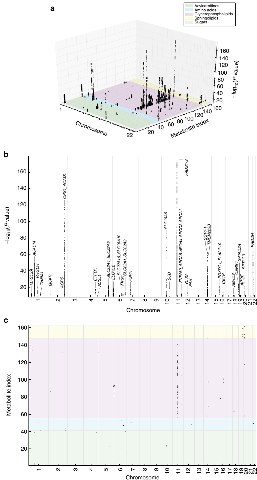
Figure 1 | Manhattan plots for all metabolites targeted by the Biocrates AbsoluteIDQ p150 kit ( N = [1,497, 7,478] ). These plots graphically display the P values for significant ( Z -test P < 1.09 \times 10^{-9} ) SNP-metabolite associations in the discovery phase in the current study. (a) A three-dimensional view; orthogonal projections are given in (b) and (c) . SNPs are arranged according to genomic location along the ‘Chromosome’ axes. The ordering of the metabolites along the ‘Metabolite index’ axes is equal in both a and c , and equal to that in Supplementary Table 3. In a and b , all data points are displayed semi-transparent and therefore opaque regions in the plot indicate clusters of significant associations. In b , loci are identified by most plausible causal gene or, if no plausible genes found, by nearest gene. Where multiple plausible genes could be identified at the locus (possibly for different metabolites), the gene names are separated by an underscore (‘_’) in the locus name. In c , the size of the markers scales linearly with -\log_{10}(P \text{ value}) . This Figure is also supplied as a movie (see Supplementary Movie 1).
