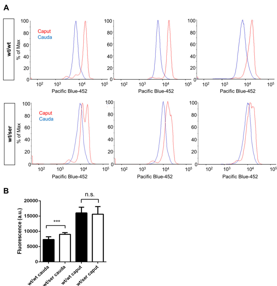
FIGURE 6. Higher levels of free thiols in cauda epididymis spermatozoa from heterozygous Gpx4 U46S mice. A, monobromobimane-labeled spermatozoa revealed an augmented fluorescence intensity signal in heterozygous animals in comparison to WT samples, whereas no detectable difference in the free thiol content was observed in spermatozoa derived from caput epididymis of both genotypes. B, a quantitative evaluation of the flow cytometry data in A revealed a statistically significant difference in free thiols between sperm samples only in those isolated from cauda epididymis (statistical analysis was conducted using t test; p < 0.001 (***)). a.u., arbitrary units. n.s., not significant.
