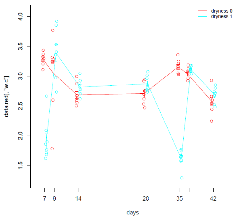
Supplementary figure 1: Variation in water contents for the different moisture regimes
