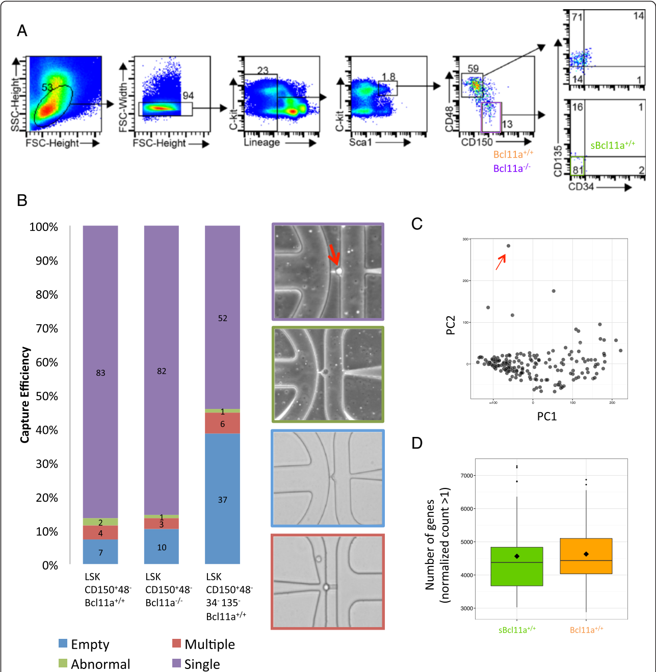
Fig. 1 Single-cell transcriptome profiling of mouse HSCs by microfluidic system. a Gating strategy for HSC purification. Bcl11a +/+ and Bcl11a -/- HSCs were isolated by sorting markers LSK CD150 + 48 - and sBcl11a +/+ HSCs by markers LSK CD150 + 48 - 34 - 135 - . Lineage markers used for enrichment included B220, CD19, CD3, CD4, CD8, TCRγδ, TCRβ, NK1.1, CD11b, Gr-1, Ter119. FSC: Forward scatter, SSC: Side scatter. b Single-cell capturing efficiency by the C1 AutoPrep microfluidic system and representative microscopic images of individual capture sites. A representative high-quality single HSC at an individual capture site is indicated by the red arrow. Representative pictures of poor quality cells, an empty capture site and a multiplet capture site are framed in colors as indicated in the key. c Principal component analysis of the transcriptome of all 181 HSCs passed initial computational quality control. One significant outlier from the Bcl11a +/+ dataset was identified (marked by red arrow). It was removed from subsequent analysis. d Boxplot comparing the number of genes detected (normalized count >1) in the sBcl11a +/+ and Bcl11a +/+ datasets. The two datasets were comparable, despite low sequencing depth of the sBcl11a +/+ dataset
