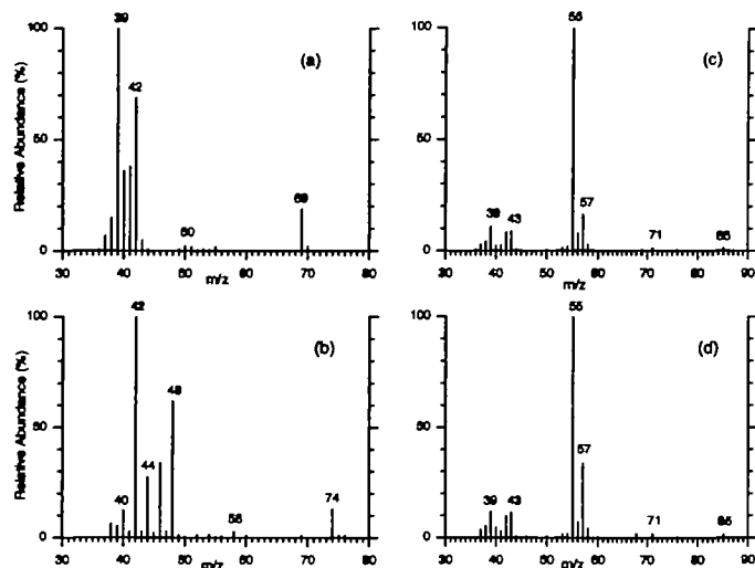
Fig. 2. Mass spectra of (a) authentic butadiene monoepoxide standard; (b) head-space sample of a reaction of B6C3F1 mouse liver microsomes with butadiene-d 6 ; (c) authentic butadiene diepoxide standard; (d) organic extract of a reaction of B6C3F1 mouse liver microsomes with butadiene monoepoxide. The incubation conditions and analytical procedures are described in the text.
