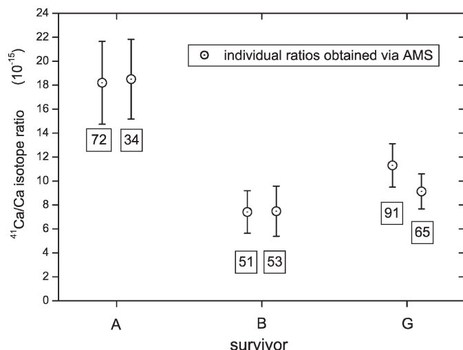
FIG. 3. Results of ^{41}\text{Ca}/\text{Ca} AMS measurements obtained from survivors who donated two teeth. The numbers in the boxes represent the sample-ID numbers in Table 5.
