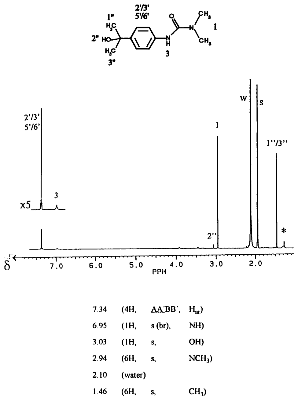
Figure 3 ^1H -NMR-spectrum and chemical shifts \delta [ppm] in CD_3CN of 2-hydroxy-isoproturon, recorded with a Bruker AC 400 spectrometer operating at 400, 13 MHz proton frequency.
