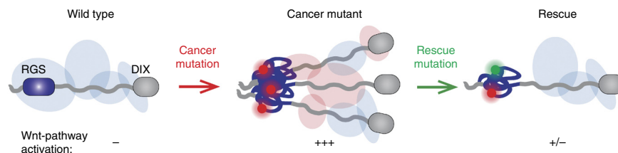
Figure 7 Model for the mechanism of action of Axin RGS cancer variants. Axin WT forms a complex with partner proteins (blue ovals) and mediates tumor-suppressor activity.
