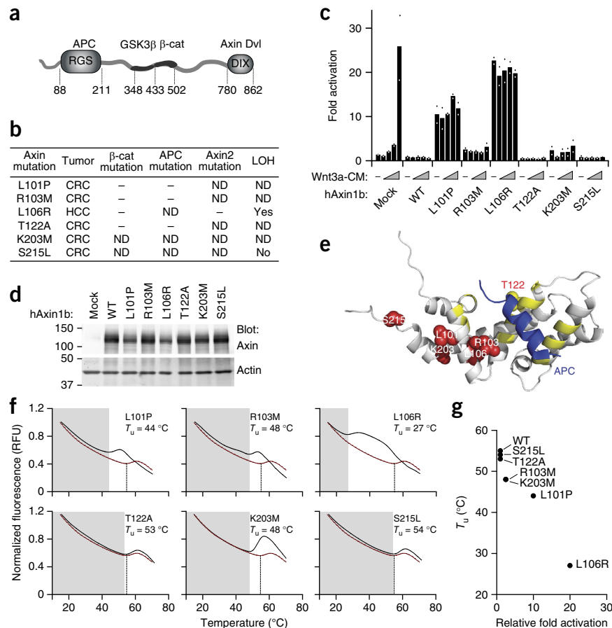
Figure 1 Axin RGS missense mutations induce Wnt-pathway activation and structural destabilization. (a) Schematic representation of full-length Axin. GSK3 \beta , glycogen synthase kinase 3 beta; \beta -cat, \beta -catenin. (b) Axin RGS-domain missense mutants identified in human tumors 20–23 . CRC, colorectal carcinoma; HCC, hepatocellular carcinoma; LOH, loss of heterozygosity; ND, not determined. (c) Wnt luciferase-reporter activity in HEK293T cells expressing mock vector, WT Axin or the indicated missense variants, and treated with increasing doses of Wnt3a-conditioned medium (Wnt3a-CM). Graph shows average (bars) and range (diamonds) of luciferase activity in duplicate cell cultures transfected in parallel. One representative experiment of three independent experiments is shown. (d) Western blot showing expression of Axin WT and the indicated Axin cancer variants. Molecular weight (kDa) is indicated at left. Actin represents a loading control. Uncropped images of blots are shown in Supplementary Data Set 1 . (e) Structure of human Axin RGS (gray) in complex with APC. Blue, APC SAMP3 peptide; yellow, APC-interacting residues; red space filling, non-APC-binding residues mutated in cancer; yellow space filling, APC-binding T122. From PDB 1EMU and 1DK8 (ref. 18). (f) Fluorescence-based thermal denaturation of WT (red dotted lines) and mutant RGS domains (black solid lines) at 340-nm emission. Results represent two independent experiments. Unfolding temperatures ( T_u ) of WT RGS (55 °C; gray boxes) and mutant Axin variants (vertical dotted lines) are indicated in each graph. RFU, relative fluorescence units. (g) Correlation graph of RGS-domain unfolding temperatures and Wnt luciferase-reporter activity observed for individual Axin cancer mutants, as indicated. The calculated Pearson correlation coefficient is r = -0.97 , P = 0.0003 (two sided; n = 7 Axin variants; correlation was calculated with values shown in c and f).
