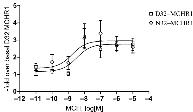
Figure 2 Functional characterization of SNP rs133072 in MCHR1 . Dose-dependent formation of IPs upon stimulation of transfected COS-7 cells with MCH. Extraction of IP from whole cell lysates was performed by Dowex chromatography. IP formation was quantified by liquid scintillation counting. The value for unstimulated D32-MCHR1-transfected cells was set at 1.0. Each point represents the means \pm S.E.M. of at least eight determinations.
