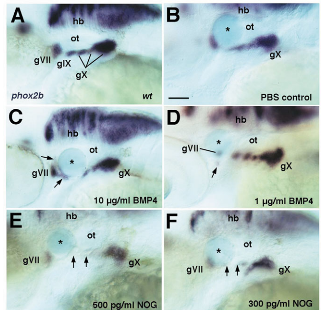
Fig. 8. BMP4-coated beads induce, and NOG-coated beads inhibit, epibranchial formation. Lateral views, anterior to the left. In situ hybridization for phox2b mRNA to label epibranchials at 48 hpf. (A) Wild-type control embryo. (B-F) Embryos that received Affi-Gel Blue beads soaked in either PBS (B), BMP4 (10 \mu g/ml, C; 1 \mu g/ml, D) or NOG protein (500 pg/ml, E; 300 pg/ml, F). Arrows in C and D indicate ectopic phox2b + cells adjacent to the bead; arrows in E and F denote missing ganglia adjacent to the NOG-coated bead. Asterisks indicate beads. gVII, facial; gIX, glossopharyngeal; gX, vagal; ot, otic vesicle. Scale bar: 50 \mu m.
