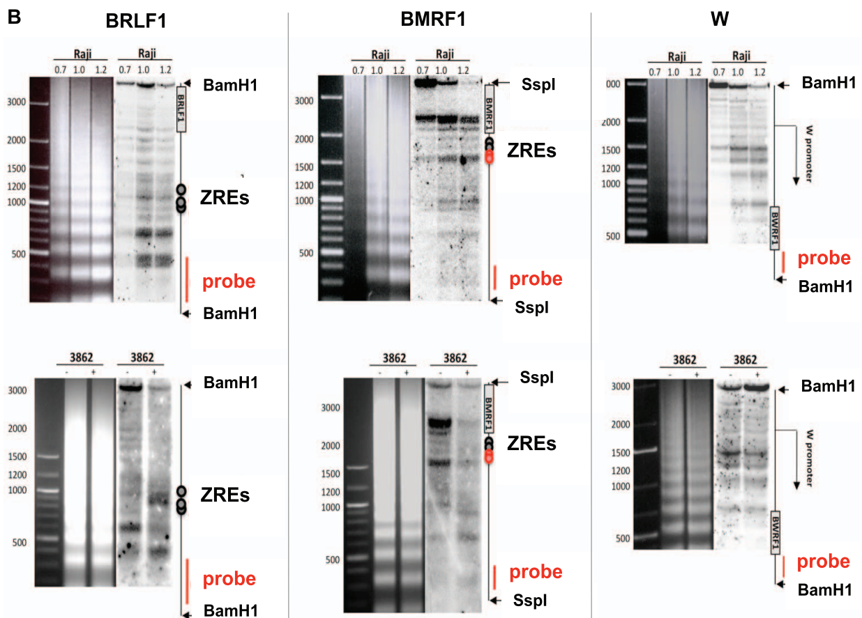
Figure 3. Chromatin Immunoprecipitation and indirect endlabeling experiments confirm the loss of nucleosomes at ZREs. (A) Chromatin Immunoprecipitation (ChIP) of histone H3. Histone H3-ChIPs confirmed the loss of nucleosomes in two promoters containing ZREs ( BRLF1 and BMRF1 ) in lytically induced cells. In contrast, the ZRE-free latent W promoter was not affected. The results of three independent experiments were averaged. Data are represented as mean \pm SD. (B) Indirect endlabeling experiments confirmed the microarray hybridization and ChIP results. Upper panels: Indirect endlabeling experiments in Raji cells are shown covering three different promoters. Lower panels: The three regions were re-analyzed in uninduced Raji-BZLF1 cells (–) or after induction with 100 ng/ml doxycycline overnight (+). The patterns in uninduced cells were similar to the ones seen in parental Raji cells. Induction of the lytic phase led to rearrangements in the nucleosomal pattern at the ZRE-containing BRLF1 promoter and the BMRF1 promoter but not in the W promoter, which lacks ZREs. doi:10.1371/journal.ppat.1002902.g003
