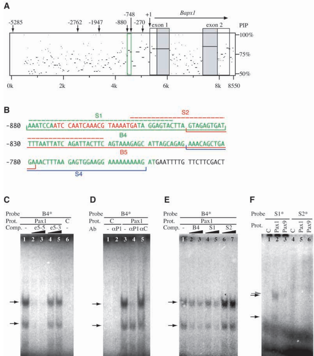
Fig. 7. Pax1 and Pax9 bind to regulatory sequences of the Bapx1 promoter. (A) PIP analysis of an 8550 bp mouse Bapx1 genome sequence when compared with an 8600 bp human BAPX1 sequence. Exons are outlined in black and coding parts are gray. Numbers at the top indicate nucleotide positions as defined in the text, and they correspond to 5' ends of intervals included in the series of deletion constructs used in the transactivation assay. The interval between -880 and -748 is outlined in green. PIP scores in % are shown on the right, with 50% identity at the bottom level. Note the presence of several CNS segments outside the coding region. Many of them are located in the interval between -880 and +109. (B) Sequence of the interval between -880 and -731. The different oligonucleotides (S1, S2, B4, B5 and S4) employed in EMSA assays are indicated by lines. Sequence in green (-880 to -748) corresponds to the segment included in the plasmid p0.9Bp-luc, but not in the plasmid p0.7Bp-luc. A potential Pax6-binding site predicted by TFSEARCH and MatInspector is in the region of S1 and indicated in red. (C-F) Results of EMSA experiments. The indicated labeled oligonucleotides (Probe, marked with an asterisk) were incubated with the in vitro translated protein (Prot.) Pax1, Pax9 or luciferase as a control (C), separated and visualized as described in the Materials and Methods. The specific Pax1 (black arrows) and Pax9 (gray arrow in F) complexes are indicated. (C) Pax1 binds to oligonucleotide B4. Cold oligonucleotides e5-5 or e5-3 were added at 250-fold (lanes 2, 4) or 500-fold (lanes 3, 5) molar excess, as indicated. e5-5 specifically competes with B4 for Pax1 binding, whereas mutated e5-3 does not. (D) Specific inhibition of Pax1-B4 complex formation by anti-Pax1 antibody. The indicated antibodies were incubated in the binding reactions. \alpha P1, anti-Pax1 goat antibody; \alpha C, anti-mouse goat antibody, used as control. The anti-Pax1 antibody abrogates the formation of the larger complex. (E) Competition experiments employing a 250-fold (lanes 2, 4, 6) or 500-fold (lanes 3, 5, 7) molar excess of cold oligonucleotides B4, S1 or S2. Note that oligonucleotides B4 and S1 compete with B4 for Pax1 binding, whereas oligonucleotide S2 does not. (F) Binding of Pax1 and Pax9 to oligonucleotide S1. S1 or S2 labeled oligonucleotides were incubated with Pax1, Pax9 or luciferase control protein as indicated. Both Pax1 and Pax9 interact with S1 oligonucleotide, but not with S2 oligonucleotide.
