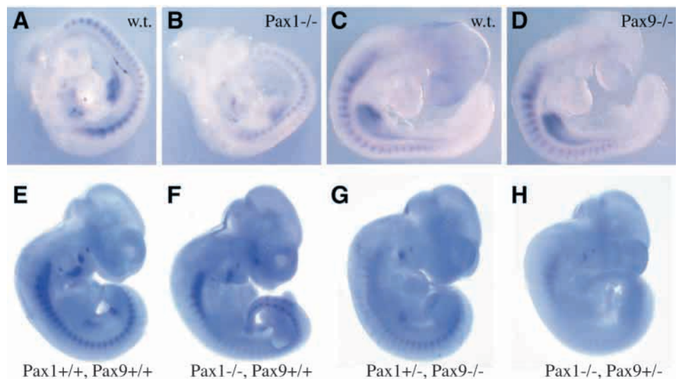
Fig. 3. Bapx1 expression level depends on the Pax1 / Pax9 gene dosage. Whole-mount in situ hybridization for Bapx1 on E9.5 (A-D) or E10.5 (E-H) mouse embryos. Genotypes are indicated on top of each panel. w.t., wild type. Note the decrease in Bapx1 staining intensity, as fewer functional copies of Pax1 or Pax9 are present.
