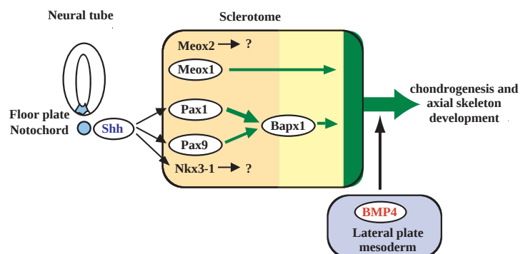
Fig. 8. Model for regulatory pathways involved in sclerotome differentiation. Ovals indicate genes with a proposed role in axial skeletal development. See text for details.
