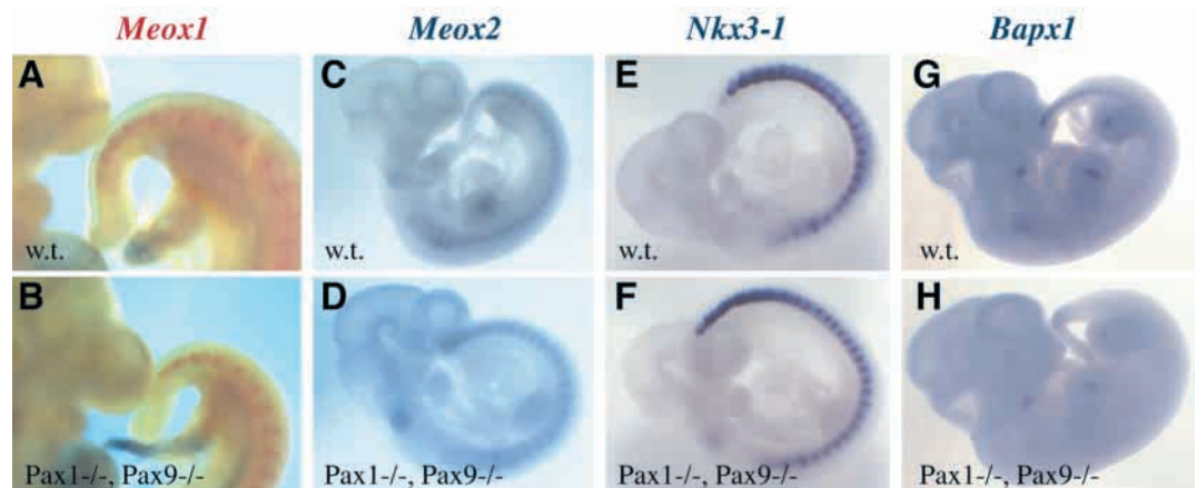
Fig. 1. Expression of sclerotomal genes in Pax1;Pax9 mutant embryos. Whole-mount in situ hybridization for Meox1 (A,B; E10.5), Meox2 (C,D; E10.5), Nkx3-1 (E,F; E9.5) and Bapx1 (G,H; E11.5) on wild type (w.t.; A,C,E,G) or Pax1 -/- , Pax9 -/- (B,D,F,H) mouse embryos.
