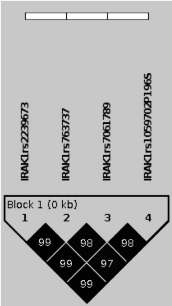
Figure 1. Schematic representation of the significant haplotype block structure in the IRAK1 gene in the French Caucasian control population. Linkage disequilibrium was measured by D' . D' values are shown within each box.
