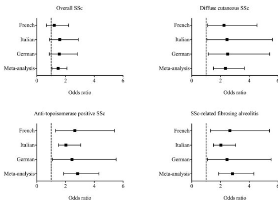
Figure 2. Meta-analysis of the IRAK1 rs1059702 TT risk genotype in 3 European Caucasian populations (French, Italian, and German). Forest plots of the meta-analysis of the association of the IRAK1 rs1059702 TT genotype with systemic sclerosis (SSc), diffuse cutaneous SSc, anti-topoisomerase I-positive SSc, and SSc-related fibrosing alveolitis in the 3 populations are shown. Bars represent the 95% confidence interval.
