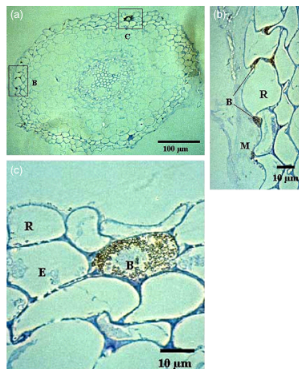
Fig. 2. (a) Light microscopic image of a root cross-section from a Miscanthus × giganteus plant inoculated with Herbaspirillum frisingense Mb11, 3 days after inoculation. Immunogold labeling with AntiMb11 and subsequent enhancement with silver staining. (b) (Detail of a) Bacterial cells (B) of H. frisingense Mb11 densely colonized the rhizoplane beneath the mucigel layer (M), penetrated the root surface and entered the intercellular spaces of the rhizodermis (R). (c) (Detail of a) An exodermis (E) is densely colonized by H. frisingense Mb11.
