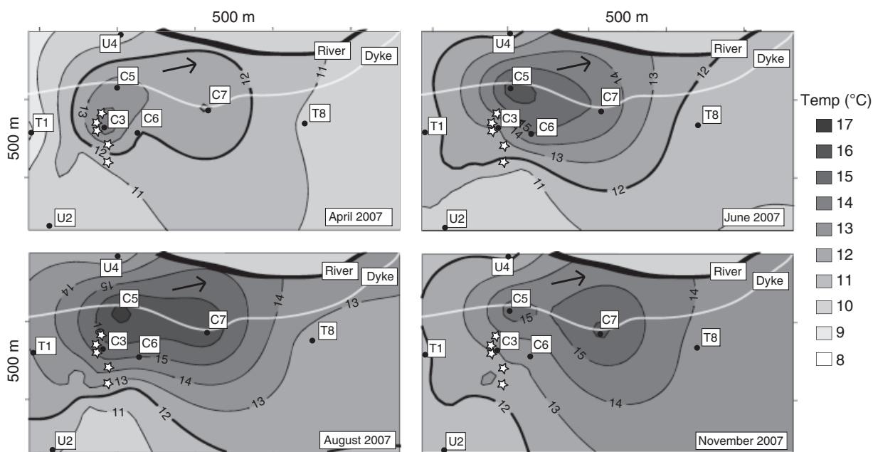
Fig. 1. Spatial dynamics of the temperature plume and location of sampling wells at the investigated field site. The extent of the plume is indicated in +1 K isotherms between 10 and 17 °C as interpolated by Kriging from the mean groundwater temperatures. Prefixes in the well names indicate unaffected (U), temporary (T) or continuous (C) temperature impacts. Stars show the location of the reinjection wells of the discharge facility; the arrow indicates the main groundwater flow direction towards the confining river.
