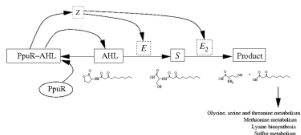
Fig. 4. Regulation pathway. The main players are shown as variables in the model approach in square boxes (AHL; AHL-PpuR complex; S , homoserines); the PpuR receptor protein, of which a constant concentration was assumed for the model, is shown in an oval. Biologically well-known components are displayed in solid boxes, hypothetical components in dashed boxes ( E , putative lactonase; E 2 , putative homoserine-degrading enzyme) and the switch variable z in a dotted box.
