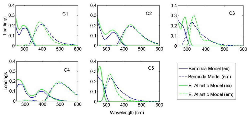
FIGURE 2 | Spectral loadings of the PARAFAC components in the Bermuda model (blue) and East Atlantic model (green).
