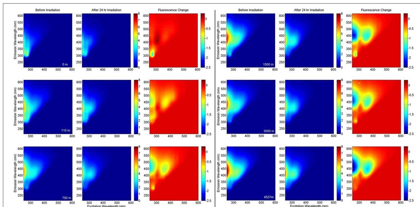
FIGURE 4 | EEM fluorescence of BATS samples at various depths before and after irradiation, and the fluorescence change. All fluorescence intensities are in Raman Units.
