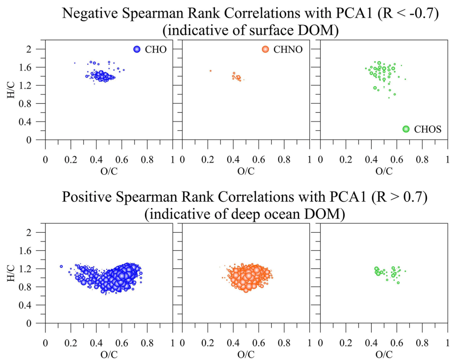
FIGURE 8 | Positive (indicative of surface DOM) and negative (indicative of deep ocean DOM) Spearman Rank correlations greater R = 0.7 and lower -0.7 , respectively of all common m/z ions, their intensities, and assigned molecular formulas with the first principal component (PCA1) derived from SPE-DOM samples collected at BATS in 2013 and analyzed by FT-ICR-MS. The bubble size corresponds to R -values between 0.7 and 1 and -0.7 and -1 , respectively.
