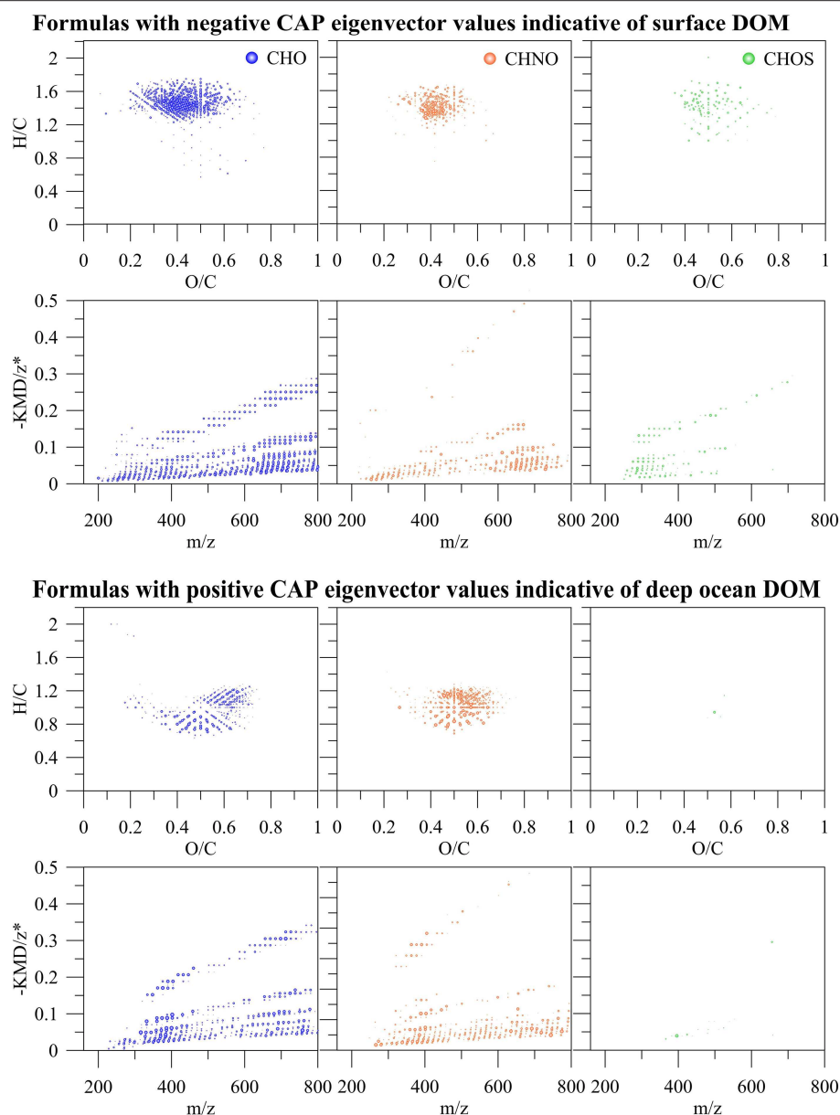
FIGURE 9 | m/z ions and associated molecular formulas with negative and positive eigenvector values of the canonical analysis on principal coordinate 1 (CAP1) of the EEM resemblance matrix and the FT-ICR-MS data of all SPE-DOM samples collected at BATS in 2013 (see also Figure 7C).
