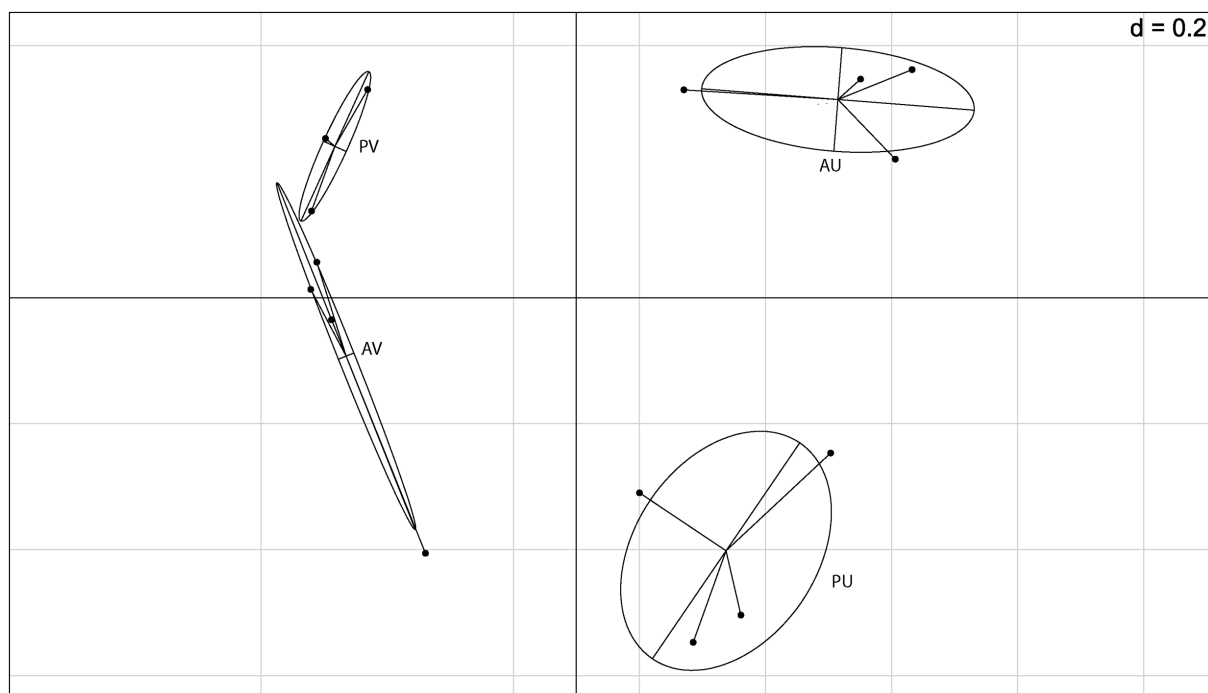
FIGURE 2 | Between group analysis (BGA) out of principal component analysis (PCA) based on 16S rRNA barcoding sequence data (OTU 5% dissimilarity). A = BRS Acauã and P = BRS Pujante, U = Ultisol and V = Vertisol.
