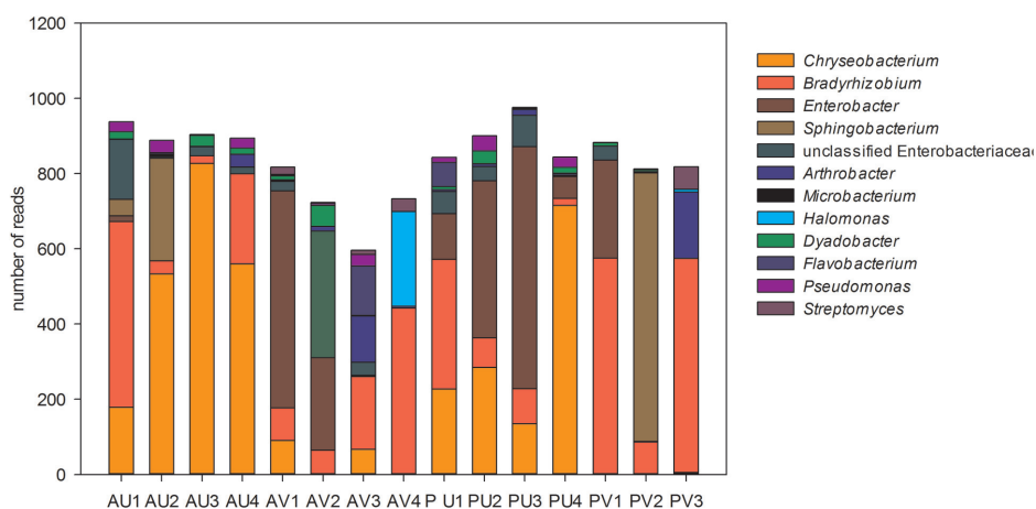
FIGURE 3 | Relative abundance (in total number of reads) of the bacterial genera present in the nodules of cowpea genotypes cultivated in different soil. Only genera that represented more than 1% of the total reads are shown.
