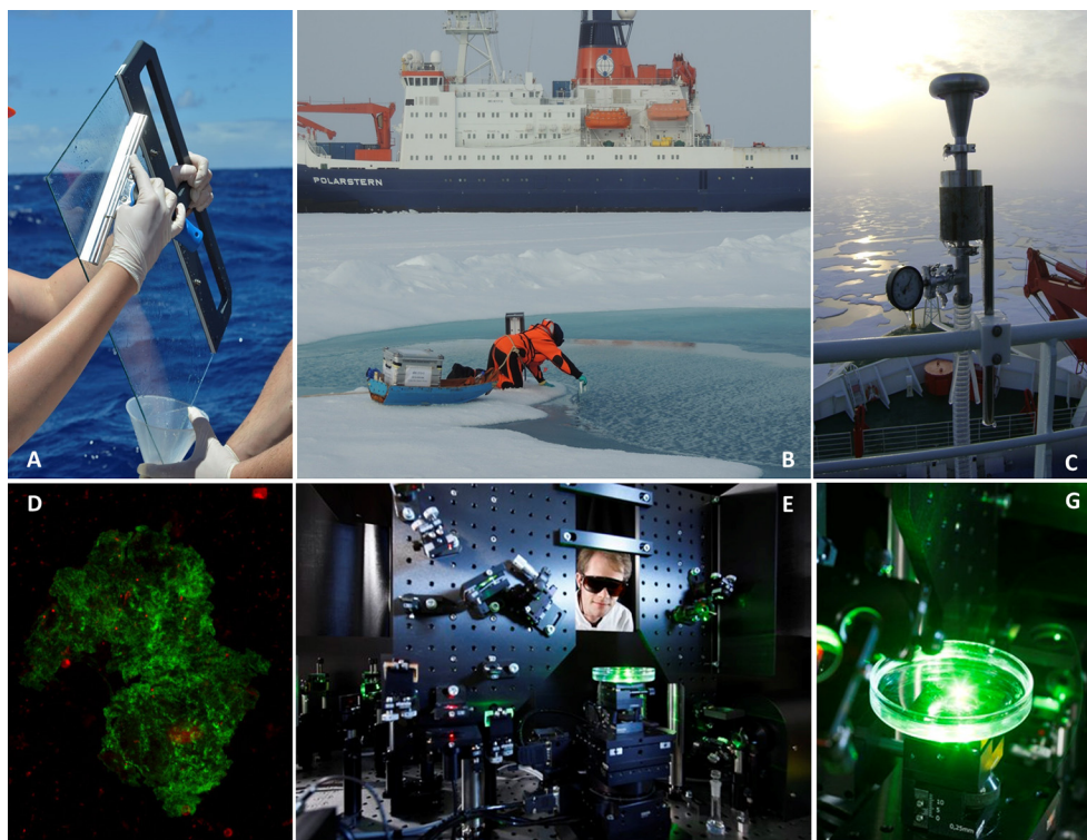
FIGURE 3 | Material accumulating in the SML can be sampled with a glass plate from the ocean ( A ) and melt ponds ( B ), or by using an aerosol collector ( C ). Advanced analysis of organic components in the SML, such as gel particles colonized by bacteria ( D ), reveal structural properties of the gelatinous SML matrix and nanolayer, which has been studied by new methods such as sum frequency generation spectroscopy (SFG) ( E,G ). Photos by: M. van Pinxteren, A. Stecher, L. Galgani, B. Zäncker, R. Frommann/Future Ocean. Written, informed consent has been obtained for the publication of images showing individuals.
