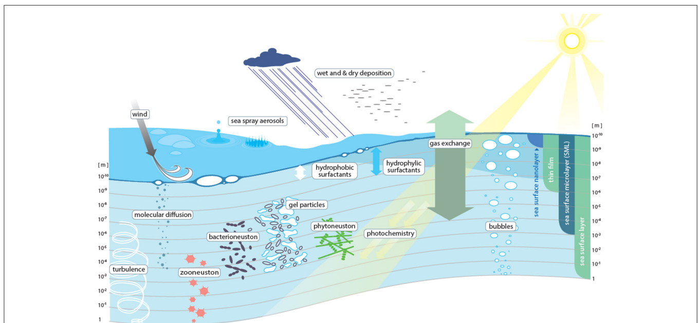
FIGURE 1 | Conceptual view of the processes determining transport across the sea surface microlayer (SML).
