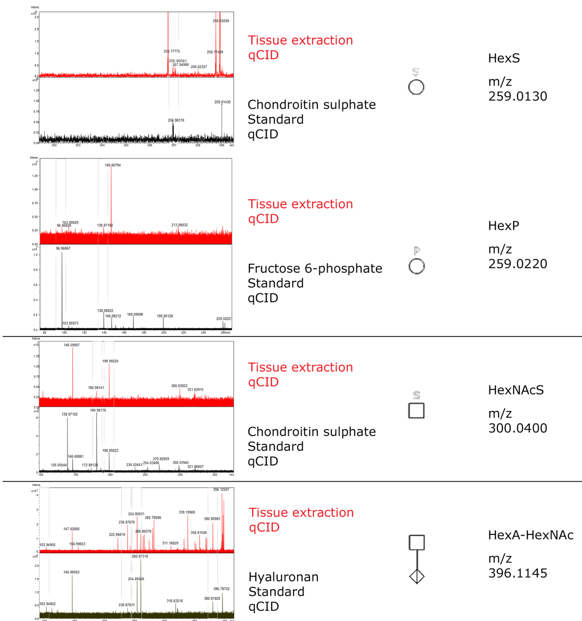
Supplementary Figure 1: Glycan validation spectra part 1: Validation spectra of HexS, HexP, HexNAcS and HexA-HexNAc.
