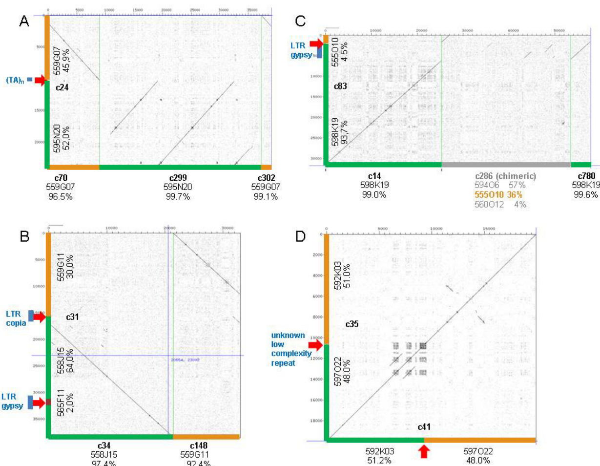
Figure 5 Sequence comparison by dotter between the chimeric contigs (y-axis) shown in Figure 4 and the corresponding contigs from the assembly of masked sequences (masked in regions with 20mer frequencies >36, m36; x-axis). (A) The two contig parts of c24, wrongly assembled at the TA-repeat are separated in m36 forming three non-chimeric contigs. (B) The misassemblies at the LTRs in c31 are not observed in the m36 assembly. (C) The misassembly at the LTR in c83 is not present in the m36 assembly. The short section from 555O10 is contained in a chimeric contig of the masked assembly (m36_c286). (D) Contig c35 is also chimeric in the masked assembly (m36_c41) with the same read fractions and >99% nucleotide identity.
