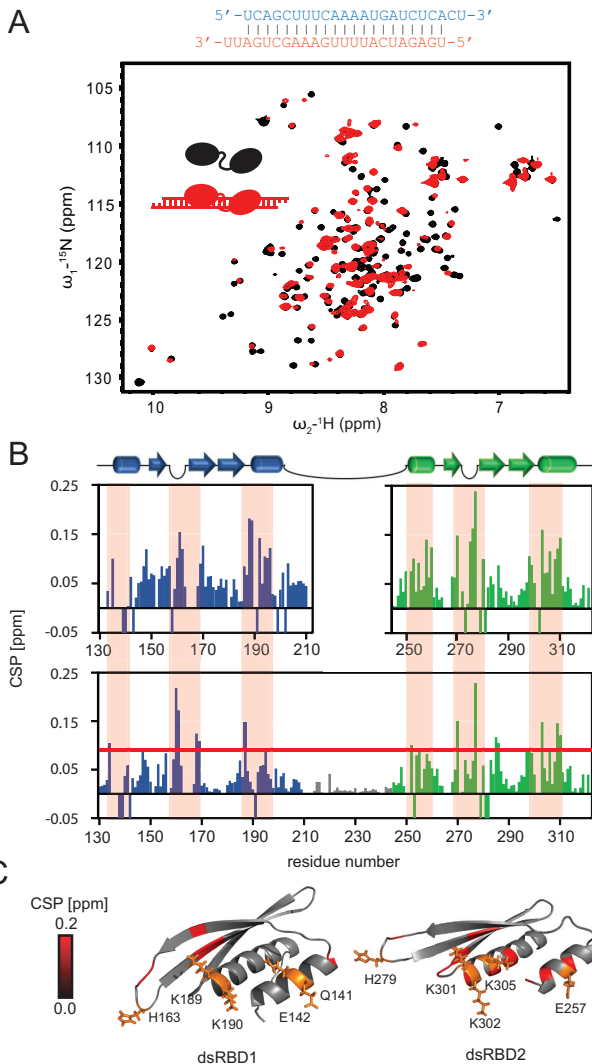
Figure 3. Loqs dsRBD1 and 2 bind siRNA independently and via conserved binding mode. (A) ^1\text{H} , ^{15}\text{N} correlation NMR spectra of Loqs-PD _{\Delta\text{NC}} free (black) and bound to ban -siRNA (red), the RNA sequence is shown above. (B) Upon titration of ban -siRNA the amide signals in the tandem dsRBD protein exhibit significant chemical shift perturbations (CSP), while the linker (gray) is not affected. The single domains titrated with the same RNA (graphs on top) show a similar pattern of CSP demonstrating that both domains bind RNA independently. Negative bars indicate broadened lines and non-traceable signals. Residues with CSP above the red line (mean \pm SD) are highlighted in C. The orange shaded boxes indicate main RNA binding regions. (C) The CSP induced by RNA binding are plotted on the domain structures and reveal three binding regions: The first helix ( \alpha_1 , \alpha_3 ), the loop ( L_1 , L_2 ) and the N terminal part of the second helix ( \alpha_2 , \alpha_4 ) are involved in RNA binding. Loqs thus binds via the typical dsRBD interface. Side chains of typical conserved RNA binding residues are shown as orange sticks. We confirmed that the Loqs dsRBD1 and dsRBD2 mediate canonical interactions with the dsRNA by similarity searches using DALI (77). Both Loqs dsRBDs superimpose well with dsRBD-dsRNA complex structures from the respective top hits (Supplementary Figure S4D, Supplementary Table S1).
