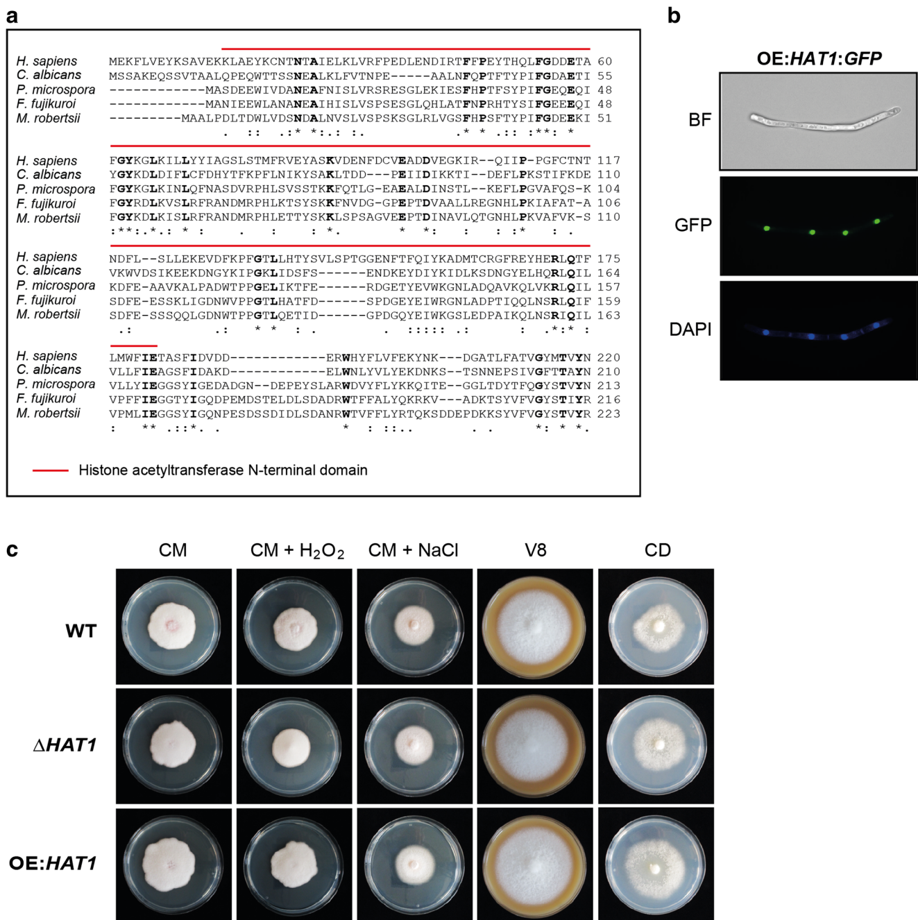
Fig. 5 Functional characterization of HAT1 in F. fujikuroi . a Multiple sequence alignment of HAT1 proteins from M. robertsii (XP_007822160.1), H. sapiens (NP_003633.1), F. fujikuroi (FFUJ_03208), C. albicans (XP_713589.1), and P. microspora (ANS59908.1) was performed using Clustal Omega (EMBL-EBI). Asterisks and dots indicate the identical and similar amino acids, respectively. b The
