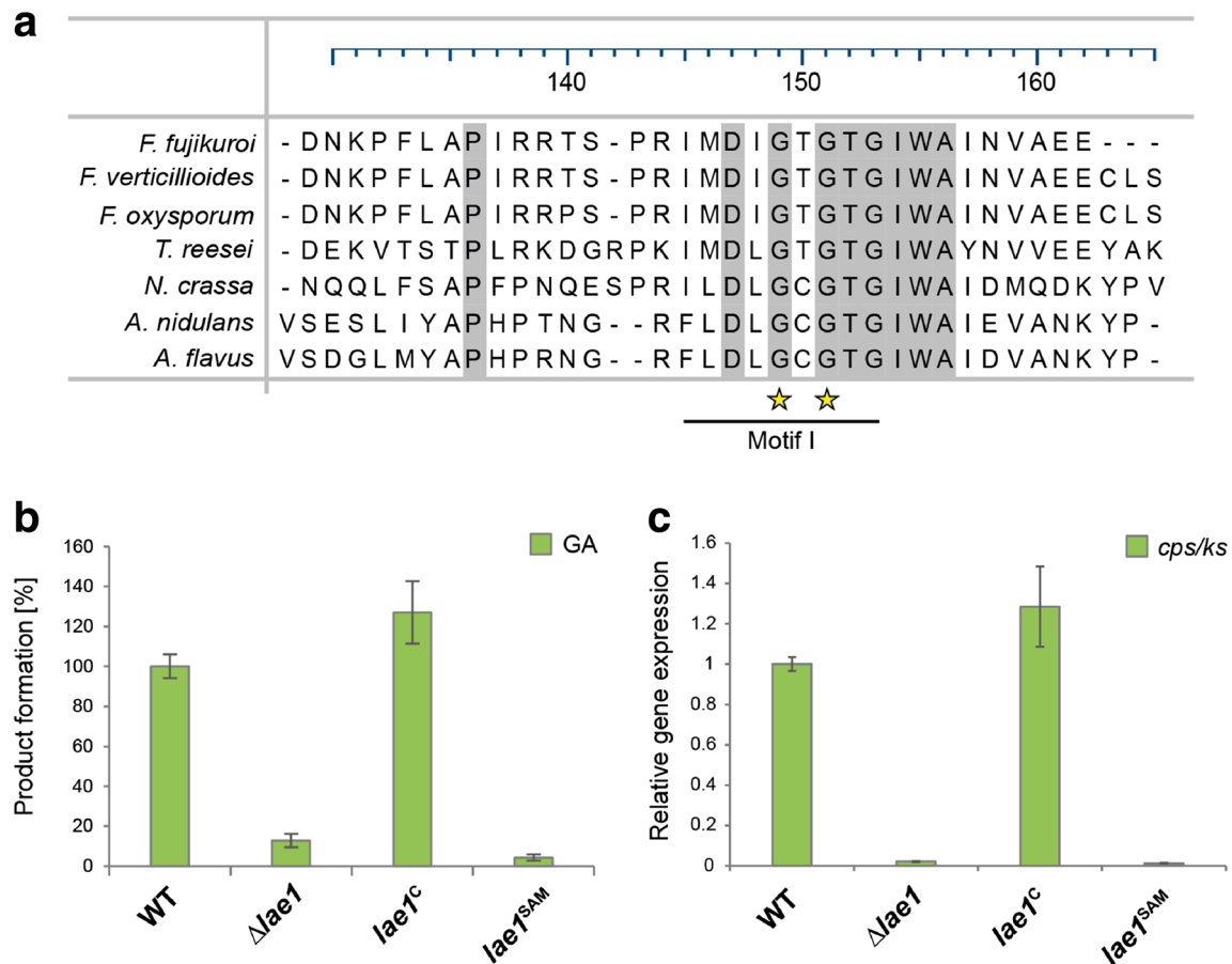
Fig. 3 The S-adenosyl L-methionine (SAM) domain of Lae1 is essential for its full activity. a Multiple sequence alignment of a part of the Lae1 SAM-binding domain from F. fujikuroi (FFUJ_00592) with characterized LaeA proteins from F. verticillioides (AHC70606.1), Fusarium oxysporum (A0A0J9UBD6), T. reesei (AFX86442.1), Neurospora crassa (ESA44297), A. nidulans (Q6TLK5), and A. flavus (AAX68412). The SAM-binding domain can be separated into four
