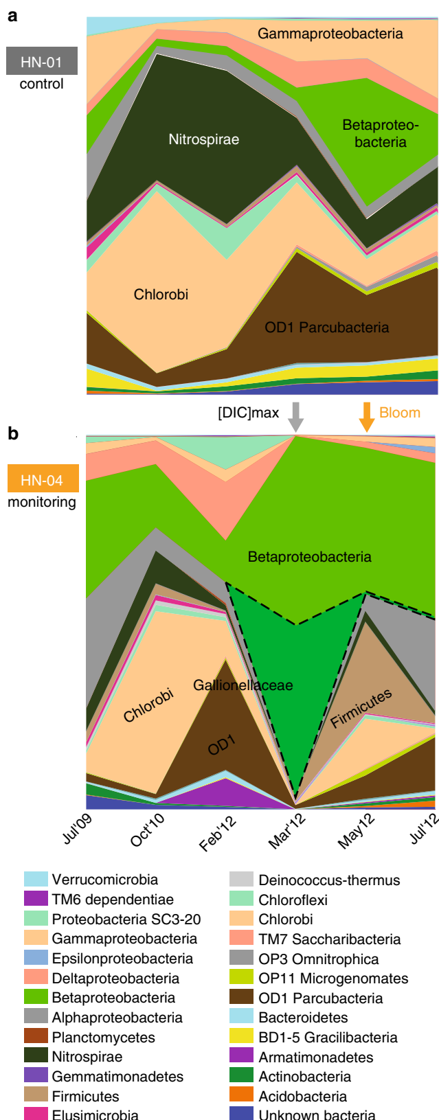
Fig. 2 Post-injection bacterial blooms based on taxonomic distribution of the 16S-rRNA gene community profile obtained from 454-pyrosequencing. The post-injection bacterial blooms are represented as a function of time in the groundwater of control well HN-01 ( a ) and monitoring well HN-04 ( b ), with colors representing different taxa. Groundwater of control well HN-01 exhibited a relatively stable bacterial community with Chlorobi, Nitrospirae, OD1 Parcubacteria and Proteobacteria as dominant community members. While broadly similar to the pre-injection community sampled from HN-01 groundwater, the HN-04 community structure was consistently different after the pure-CO 2 injection. In particular, growth of Betaproteobacteria accounting for 88% of the community in March 2012, was first favored; note a bloom of Gallionellaceae related species, which were only weakly detected before the injection (similarly shown by metagenomic analysis; Supplementary Fig. 10). It was followed by Firmicutes accounting for more than 20% of the groundwater community in May 2012, hence dominating with betaproteobacterial Thiobacillus species (Supplementary Fig. 10)
