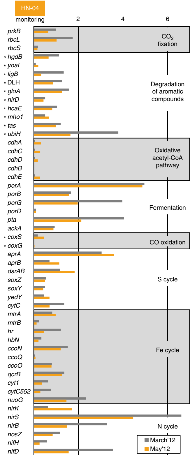
Fig. 6 Normalized counts of key biomarkers in groundwater from monitoring well HN-04 sampled in March and May 2012. prkB phosphoribulokinase, rbcL-S ribulose 1,5-bisphosphate carboxylase, large and small subunits, hgdB benzoyl-CoA reductase, yoal aromatic ring hydroxylase, ligB aromatic ring-opening dioxygenase, DLH dienelactone hydrolase, gloA catechol 2,3-dioxygenase, nirD ring-hydroxylating dioxygenase, hcaE phenylpropionate dioxygenase or related ring-hydroxylating dioxygenase, mho1 predicted class III extradiol dioxygenase, tas predicted oxidoreductase, ubiH 2-polyphenyl-6-methoxyphenol hydroxylase, cdhA-E CO dehydrogenase/acetyl-CoA synthase subunits, porA-D pyruvate:ferredoxin oxidoreductase or related 2-oxoacid:ferredoxin oxidoreductase subunits, pta phosphotransacetylase, ackA acetate kinase, coxS-G aerobic-type carbon monoxide dehydrogenase subunits, aprA-B adenylyl sulfate reductase, dsrAB sulfite reductase, dissimilatory type, soxZ-Y sulfur oxidation protein, yedY sulfite oxidase, cytC sulfite dehydrogenase, mtrA MR-1 decaheme cytochrome, mtrB decaheme cytochrome, hr hemerythrin, hbN truncated hemoglobin, ccoN-O cbb3-type cytochrome oxidase subunits, qcrB cytochrome b subunit of the bc complex, cyt1 cytochrome c1, cytC552 cytochrome c551/c552, nuoG NADH dehydrogenase/NADH/ubiquinone oxidoreductase, nirK copper containing nitrite reductase, nirS cytochrome cd1 containing nitrite reductase, nirB Nad (P)H-nitrite reductase, nosZ nitrous oxide reductase, nifH-D nitrogenase subunits. When relevant, aerobic and anaerobic pathways are indicated by a circle and a star, respectively (see Supplementary Table 7). Note that ubiH could also be involved in the synthesis of ubiquinone used in conjunction with the bc1 cytochrome for iron oxidation in Sideroxydans sp 22
