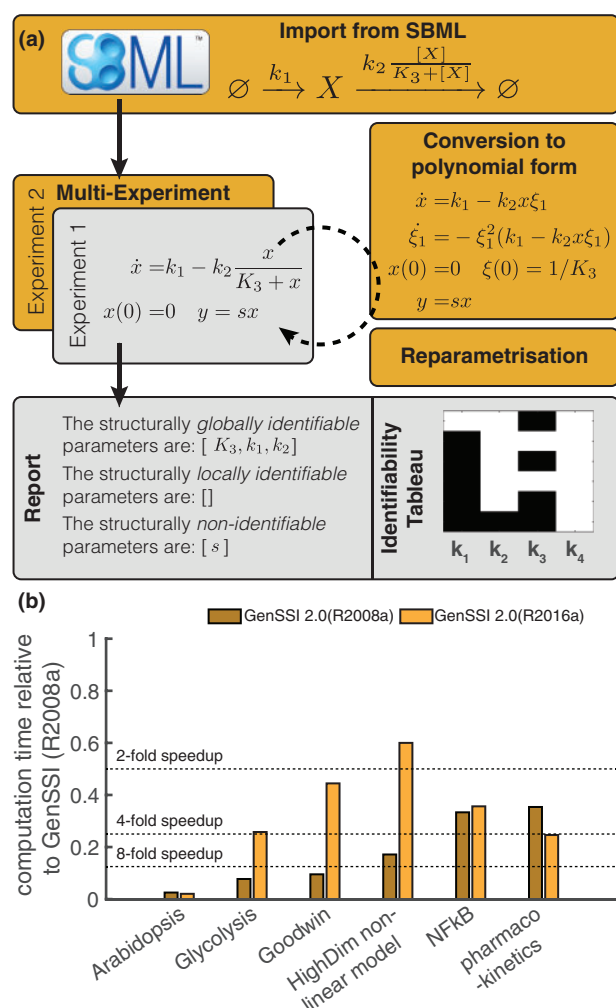
Fig. 1. Properties of GenSSI 2.0. (a) Features implemented in GenSSI 2.0. Novel features are indicated in dark tone. (b) Performance evaluation of GenSSI and GenSSI 2.0 on different MATLAB versions
