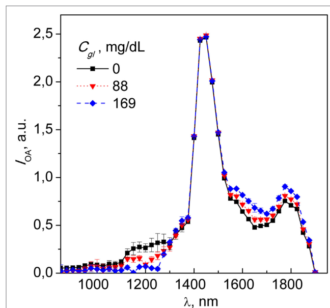
FIGURE 2 | Spectra of distilled water with subsequent glucose titrations at 88 and 169 mg/dl; each spectral point represents an average of five independent readouts, with error bars indicating the SD of the optoacoustic signal. Note the dose-dependence diversion of the spectra of glucose-containing analyte from that of DH_2O .
