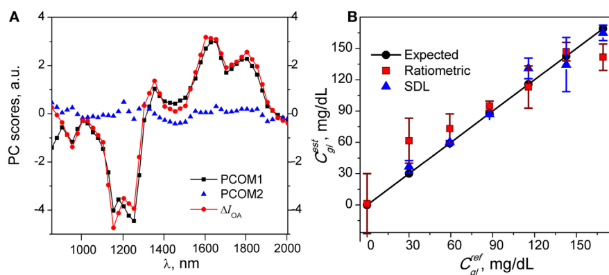
FIGURE 4 | (A) Scores of PCA component (PCOM1) (black squares) and PCOM2 (blue triangles) of principal component analysis of the optoacoustic spectroscopy (OAS) of glucose. For illustration purpose, PCOM readouts are overlaid with near-infrared-optoacoustic spectroscopy (NIR-OAS) \Delta I_{OA} (red circles) of 169 mg/dl glucose solution is also plotted on Figure 4A . The variance of the first PCA component (PCOM1) accounts for \sim 96.6\% of total variation, while PCOM2 accounted for a negligible \sim 1.6\% variation. PCOM3 (not shown) offered \sim 0.8\% variation and subsequent components were negligible. PCOM1 is found to faithfully follow the \Delta I_{OA} trajectory shown in Figure 3A , while the data points of PCOM2 appear to have random values and possibly reflect systematic errors in the measurement ( Figure 4A ). This observation and the calculated SDs of components indicate that only PCOM1 was significant for glucose measurements. Unidimensional composition of the titration dataset indicates that under our settings, within investigated concentration ranges,
