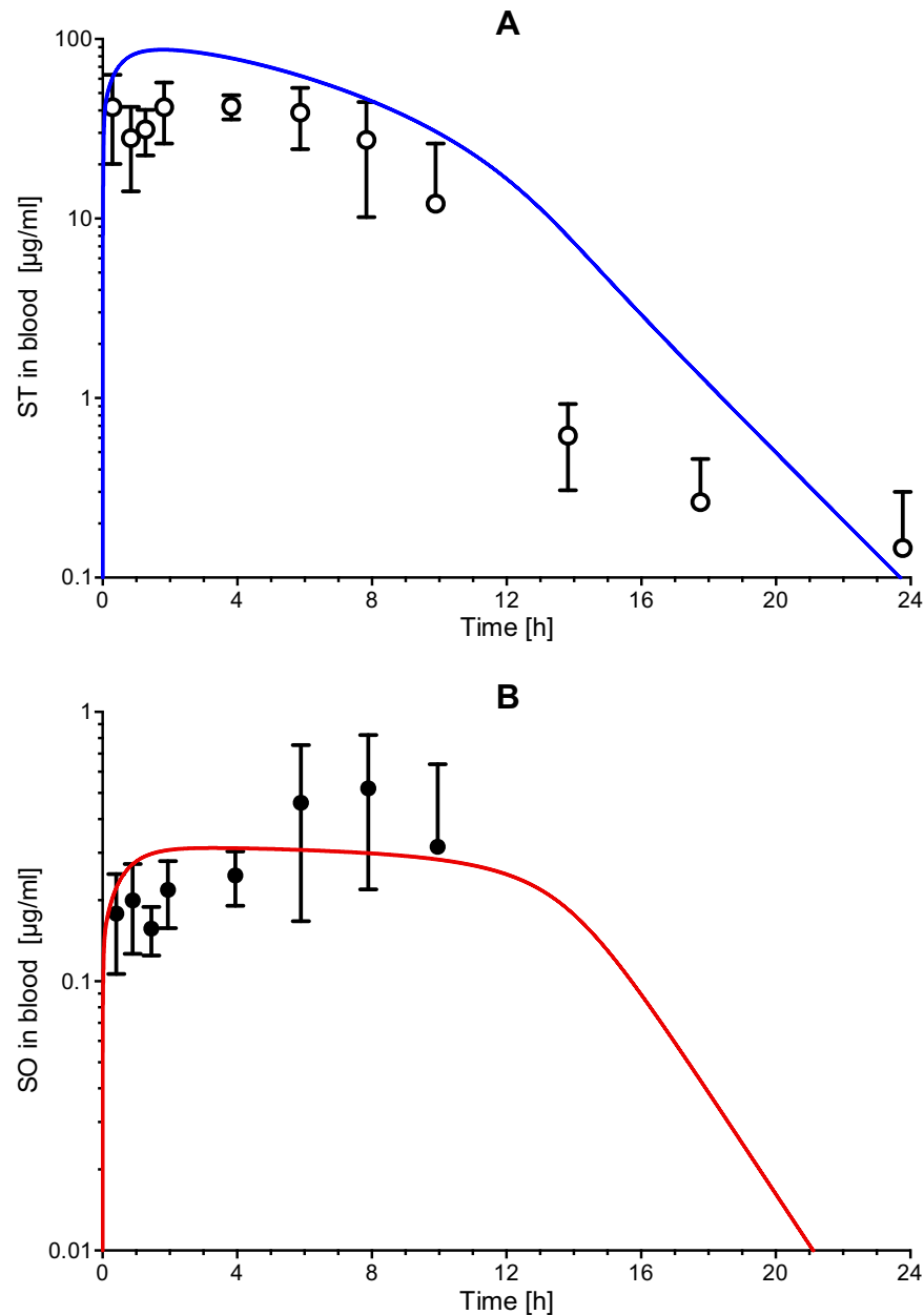
Fig. 3. Concentration-time courses of styrene (ST, A) and styrene-7,8-oxide (SO, B) in blood of male F344 rats after oral administration of 500 mg ST/kg BW. Measured data (ST: ○ SO: ●) ±SDs from Mendrala et al. (1993). Minus SDs that were smaller than the smallest value on the y-axis are not shown. The limit of quantification of SO was 0.010 µg/ml blood. The curves were predicted by the PT model for a rat with a BW of 174 g, the average of the BWs of the rats used by Mendrala et al. (1993).
