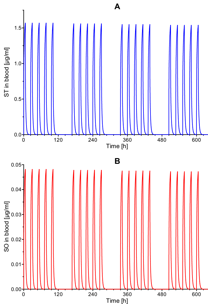
Fig. 5. PT-model-calculated concentration-time curves of styrene (ST, A) and styrene-7,8-oxide (SO, B) in venous blood of a male F344 rat exposed repeatedly (6 h/d, 5 d/w, 4 w) by inhalation to vaporous ST at a concentration of 75 ppm (according to the experimental design of Gaté et al., 2012). At the start of the study, the rat was 6 w old. BW was set to 130 g, 157 g, 184 g, and 211 g for the first, second, third, and fourth week of exposure, respectively.
