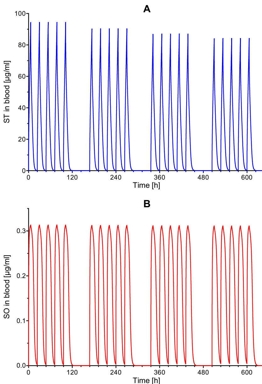
Fig. 6. PT-model-calculated concentration-time curves of styrene (ST, A) and styrene-7,8-oxide (SO, B) in venous blood of a male F344 rat exposed repeatedly (6 h/d, 5 d/w, 4 w) by inhalation to vaporous ST at a concentration of 1000 ppm (according to the experimental design of Gaté et al., 2012). At the start of the study, the rat was 6 w old. BW was set to 130 g, 157 g, 184 g, and 211 g for the first, second, third, and fourth week of exposure, respectively.
