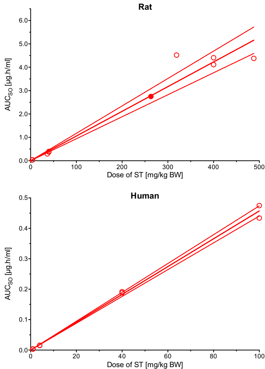
Fig. 12. Daily areas under the PT model-calculated concentration-time curves of styrene-7,8-oxide (SO) in venous blood ( AUC_{SO} ) of male and female rats and of humans versus the doses of styrene (ST) taken in. Data points (10 for male rats, 1 (full symbol) for female rats, and 9 for humans; some not visible because of overlapping) were taken from Table 3. Curves are linear regression lines through the origin \pm 95% confidence bands of the fitted lines. The slopes m of the linear functions ( AUC_{SO} = m \times \text{dose of ST} ) and their standard errors are m = 0.01057 \pm 0.000520 ( \mu\text{g SO} \times \text{h/ml} )/(mg ST/kg BW) in rats and m = 0.00457 \pm 0.0000728 ( \mu\text{g SO} \times \text{h/ml} )/(mg ST/kg BW) in humans. The coefficients of determination ( r^2 ) are 0.9533 (rats) and 0.9966 (humans).
