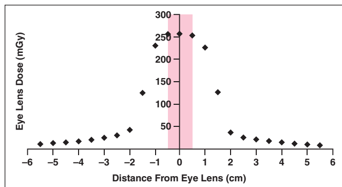
Fig. 4 —Graph shows eye lens dose as function of scanning location from protocol of American Association of Physicists in Medicine (80 kVp, 24 \times 1.2 -mm collimation, 270 mAs/rotation, 40 rotations) for brain perfusion CT examination using Sensation 64 scanner (Siemens Healthcare). Width of eye lens in z direction for this patient model (Irene, GSF [now Helmholtz Zentrum München]) is 1 cm. Shaded box indicates eye lens range in longitudinal direction. Therefore, when scanning location is 2 cm from center of eyes, eye lenses are completely out of x-ray beam (larger than half of beam width plus half of eye lens width).
