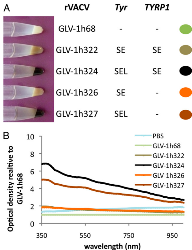
Fig. 1. Production of melanin upon key enzyme expression. ( A ) Pellets of infected CV-1 cells and overview of the infecting rVACV strains encoding Tyr and/or Tyrp1 under control of a weaker SE or strong SEL promoter. The colored dots indicate the color used for each strain in all following figures. ( B ) Optical density measurements over the spectrum from 350 nm to 1,000 nm (in 5-nm increments) were conducted, and the relative optical density compared with the results obtained with GLV-1h68 infected A549 cells was plotted for each data point.
