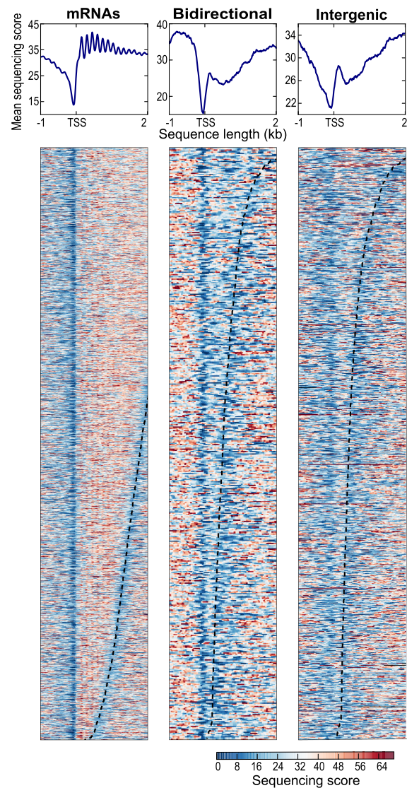
FIGURE 7. Nucleosome patterns for coding and noncoding transcribed regions. Nucleosome profiling data for all mRNA loci ( left ), 509 bidirectional lncRNA loci, and 1119 intergenic lncRNA loci ( right ) in proliferating wild-type cells. Bidirectional lncRNA loci that overlap mRNAs in antisense direction were not included. We omitted 70 intergenic lncRNA loci that showed unusually high histone occupancies (Supplemental Table S8); these loci are mostly located in centromeric or subtelomeric regions. The top graphs show average nucleosome profiles for the different types of transcribed regions, aligned to the transcription start sites (TSS). The lower graphs show heatmaps for the first two kilobases of all transcribed regions analyzed, ordered by transcript length from top (longest RNAs) to bottom (shortest RNAs). Sequencing scores are color-coded as shown in legend at bottom right .
