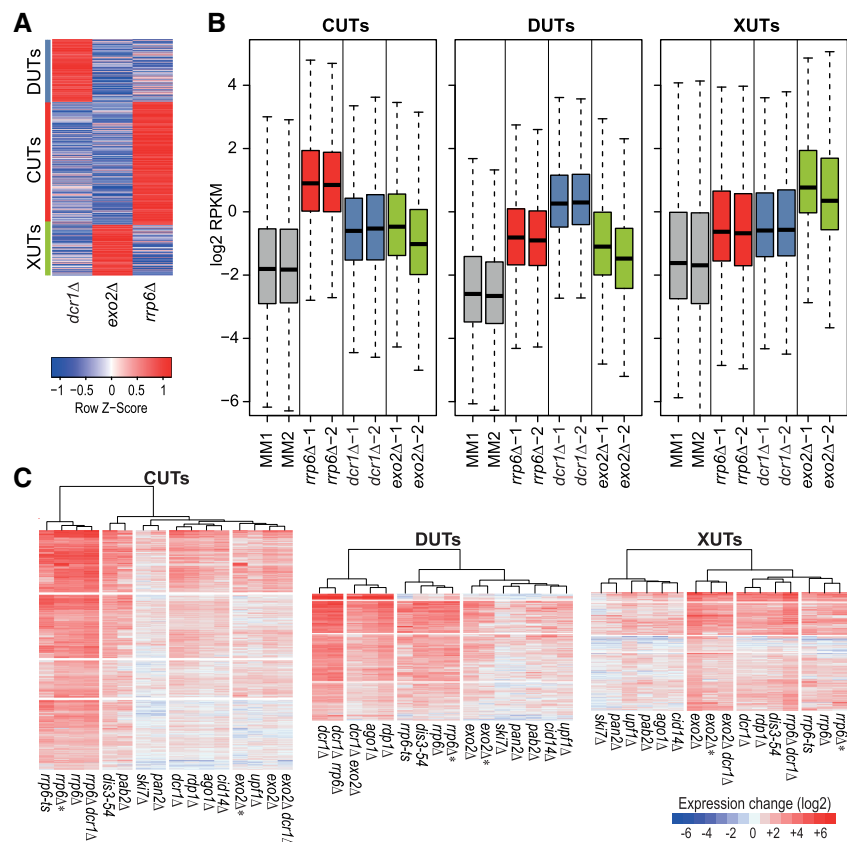
FIGURE 4. Classification of lncRNAs into CUTs, DUTs, and XUTs. (A) The lncRNAs significantly induced (DESeq2; adjusted P \leq 0.05 ) in rrp6Δ , dcrl1Δ , or exo2Δ mutants were clustered into CUTs, DUTs, and XUTs, respectively, using the Mfuzz R package (default parameters, three clusters specified). The clustering shows the 5586 uniquely classified lncRNAs after filtering those with a membership score < 0.7 . The red/blue colors indicate the mean RPKM values in the three mutants as indicated, scaled by subtracting the mean of the row and division by the standard deviation of the row ( z -score). The assigned clusters are indicated at left. (B) Box plots of RPKM values ( \log_2 ) of all CUTs (left), DUTs (middle), and XUTs (right) in control (MM) and mutant cells as indicated. The data for the biological repeats 1 and 2 are plotted separately. (C) Hierarchical clustering of genetic conditions for all CUTs, DUTs, and XUTs as indicated. Changes in RNA levels in response to the different genetic conditions (indicated at bottom) relative to control cells grown in minimal medium are color-coded as shown in the legend at bottom right ( \log_2 expression ratios). All expression and classification data are provided in Supplemental Table S3.
