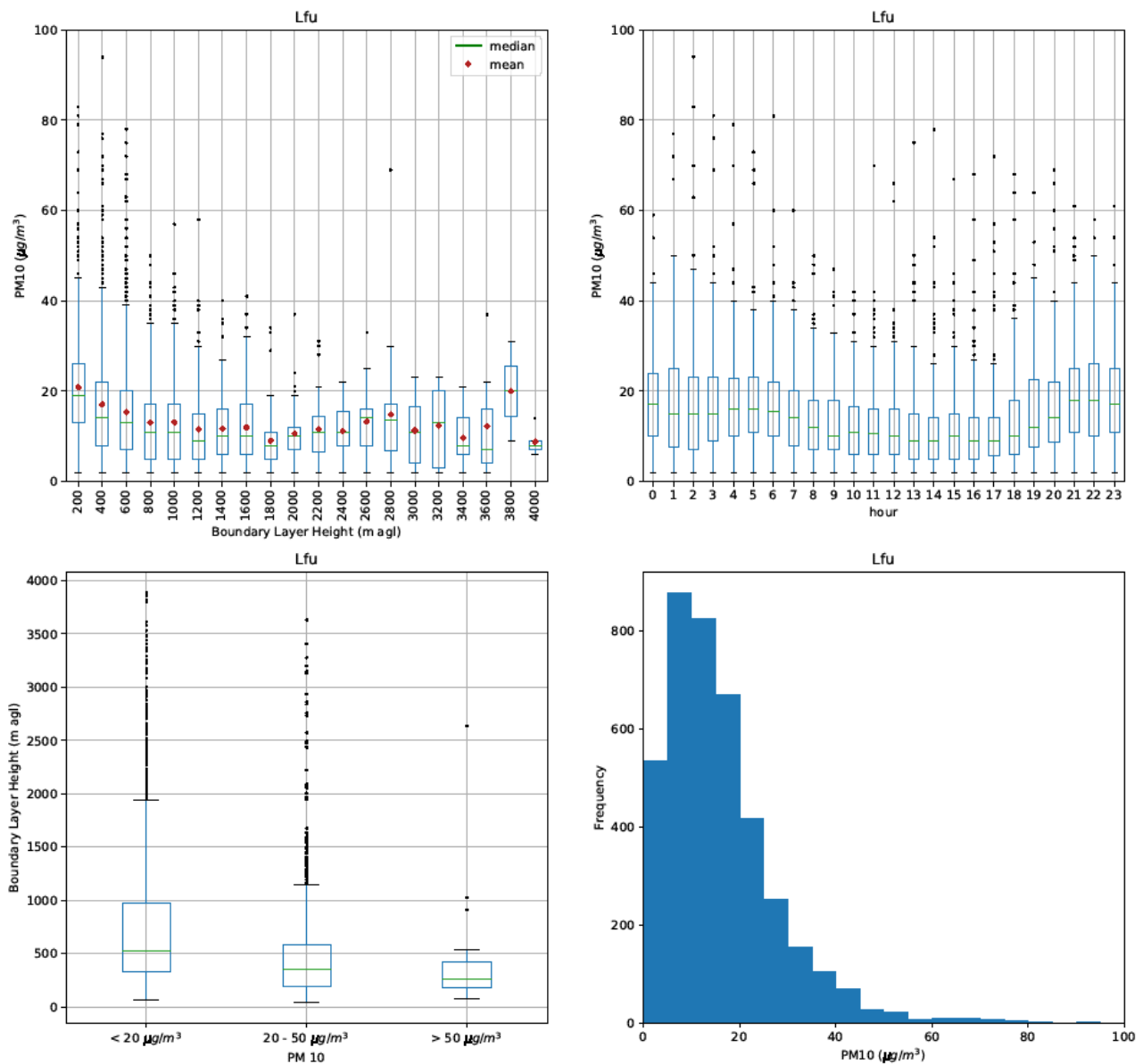
Figure 9: Analyses of the PM 10 concentration data at the LfU station (urban background) together with boundary layer height (BLH). Top left: PM 10 concentrations for different BLH, divided into 200 m intervals. Top right: Boxplot of the daily course of PM 10 concentrations in one-hour intervals. Bottom left: Boxplot of the BLH grouped into three categories of PM 10 concentrations. Bottom right: Histogram of PM 10 concentrations in 5 µg/m 3 intervals.
