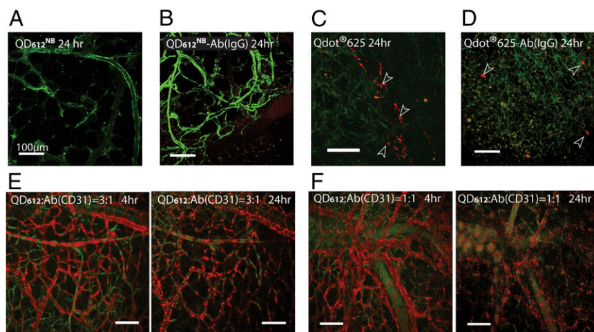
Fig. 3. In vivo microscopy imaging of blood vascular endothelial cells using QD-Ab conjugates. (A–D) Imaging of nonspecific binding for (A) QD 612 NB , (B) QD 612 NB -TzAb(IgG), (C) Qdot 625 (commercial), and (D) Qdot625-Ab(IgG) (commercial). QD 612 NB and QD 612 NB -TzAb(IgG) display virtually no nonspecific binding, whereas commercial Qdot 625 and Qdot625-Ab(IgG) show significant nonspecific binding. (E and F) Labeling of endothelial cells using the QD 612 NB -TzAb (CD31). Images taken at 4 and 24 h after the injection of QD 612 NB -TzAb(CD31) synthesized at QD:Ab ratios of (E) 3:1 and (F) 1:1 show that QD 612 NB -TzAb(CD31) with different ratios specifically labeled the GFP + vascular endothelium from 3 to 4 h up to 24 h after systemic injection. Green and red signals represent fluorescence from GFP + vascular endothelium and QDs, respectively.
