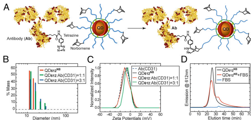
Fig. 1. \text{QD}^{\text{NB-TzAb}} nanoconjugate synthesis and characterization. (A) Conjugation of QDs to Abs. Ab (IgG 2a ) is used to represent the Ab, and Lys residues of Ab(IgG 2a ) are marked in red. This diagram is not to scale. (B) Dynamic light scattering data of the QDs and the \text{QD}^{\text{NB-TzAb}} illustrate that \text{QD}^{\text{NB}} /Ab conjugation does not yield noticeable aggregates and that the size of \text{QD}^{\text{NB-TzAb}} is compact. (C) \zeta -Potential measurements of the QDs and the \text{QD}^{\text{NB-TzAb}} show that the surface charge of \text{QD}^{\text{NB}} and \text{QD}^{\text{NB-TzAb}} is moderately negative. (D) Gel filtration chromatography (GFC) traces of \text{QD}_{612}^{\text{NB}} before and after serum incubation show that there is virtually no nonspecific binding of \text{QD}^{\text{NB}} to serum proteins.
