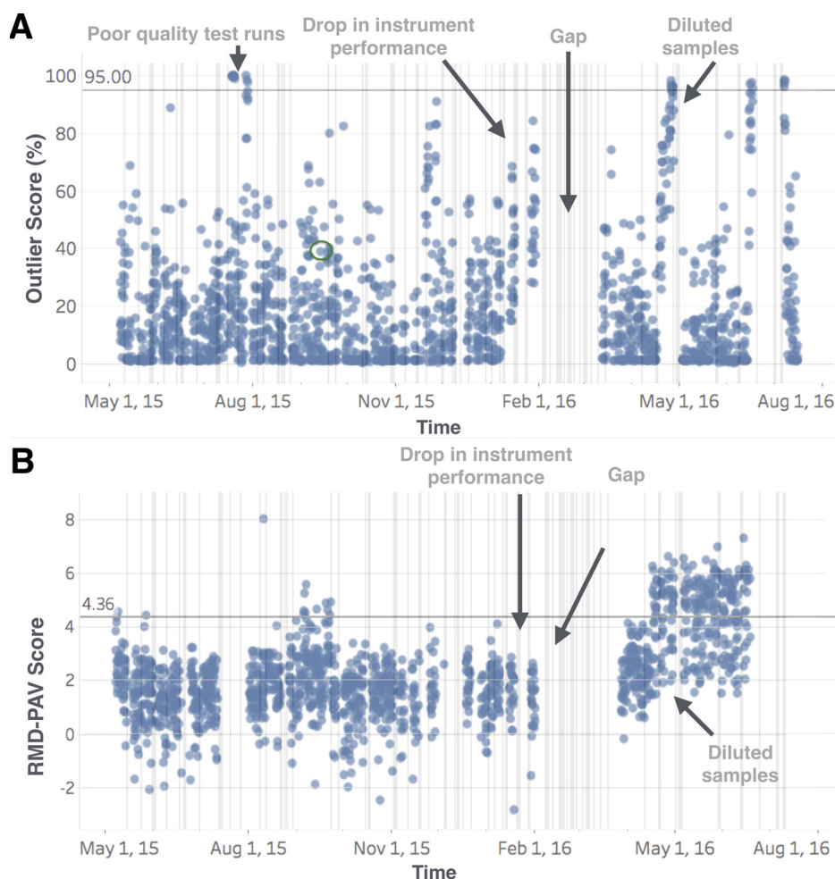
FIG. 4. Results of the InSPECTor and RMD-PAV methods for the TEDDY iTRAQ data with labeled time periods of interest. A, The InSPECTor outlier scores (%) were computed using a neighborhood size of 10 and are plotted for each instrument run in chronological order. The horizontal line corresponds to a 95% threshold and the green point represents a sample that exhibited suspicious oxidation patterns. The mistuned sample runs and some of the diluted samples were correctly flagged to be of poor quality, but the instrument drift was not detected. B, The RMD-PAV scores were computed for each fraction set once. The solid horizontal line corresponds to a 99.9% threshold. Some of the diluted samples were correctly flagged to be of poor quality, but the large shift in instrument performance at the end of the cohort prevents RMD-PAV from identifying many of the other phenomena of interest during this study.
