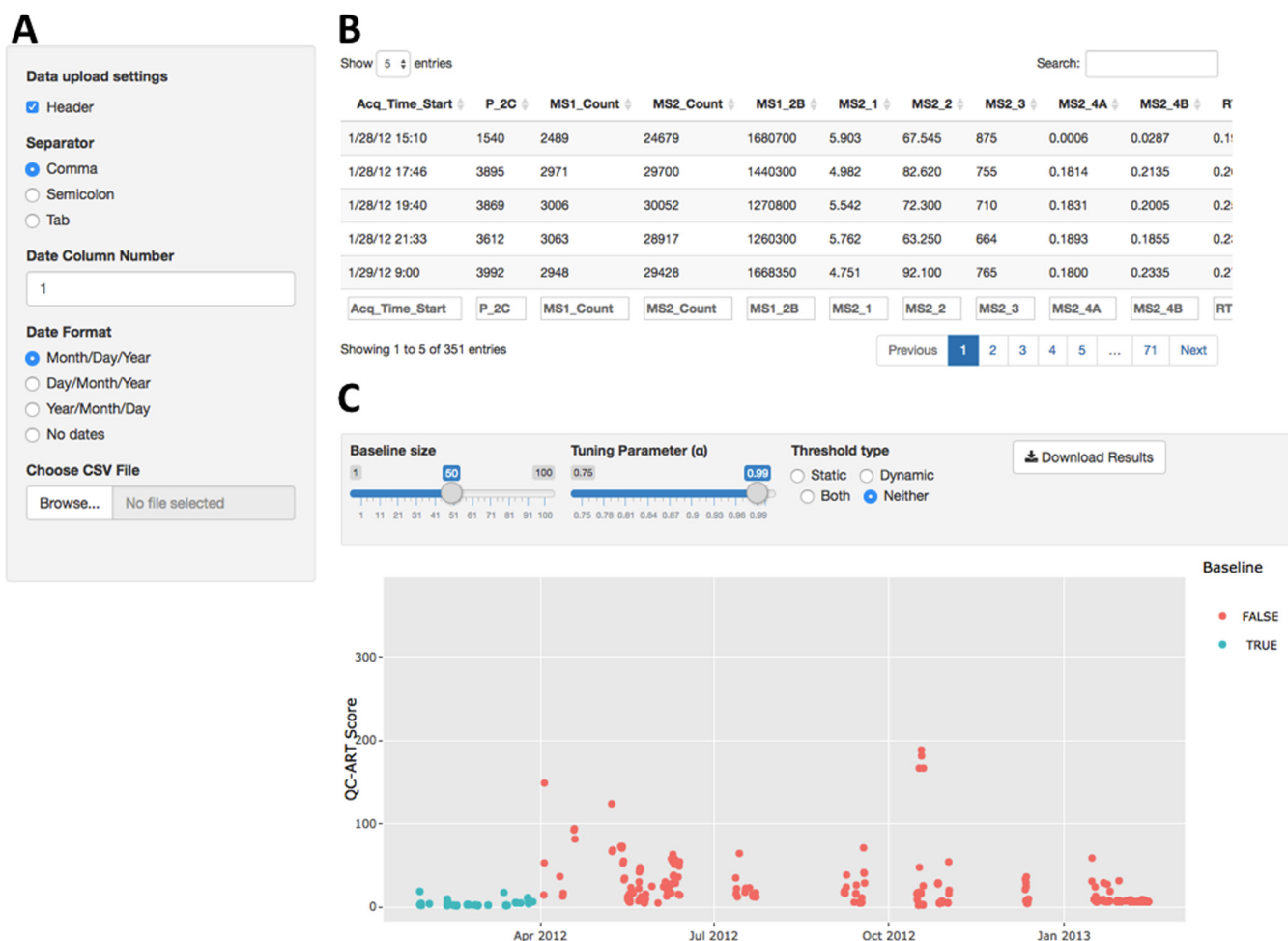
Fig. 6. QC-ART interface. A, Data upload and settings. B, Verification of the uploaded data. Once the data are uploaded they can be verified and searched. C, Results and output. The results can be visualized in the interactive graph and downloaded as a comma separated file. Tuning parameters, including baseline size, can be adjusted by experienced users to better discriminate poor-quality runs.
