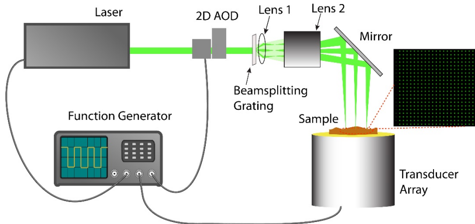
Fig. 1 Schematic drawing of the system setup.
