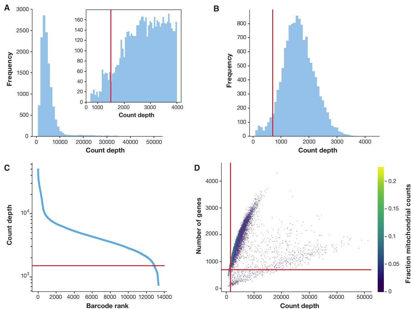
Figure 2. Plots of quality control metrics with filtering decisions for a mouse intestinal epithelium dataset from Haber et al (2017).
