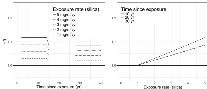
Fig. A5 Selected lag response curves of the hazard ratio (HR) for exposure rates between 1 \frac{mg}{m^3} and 5 \frac{mg}{m^3} (left panel) and exposure response curves for time since exposure between 10 yr and 30 yr (right panel) for silica dust for the preferred DLNM NL4.
