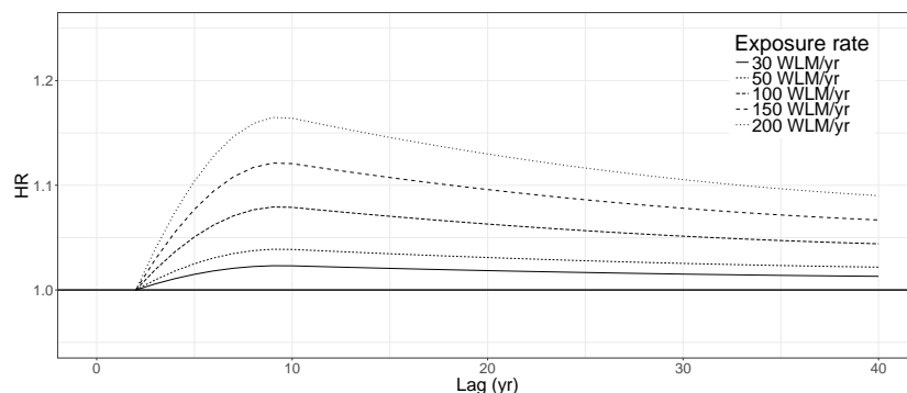
Fig. A2 Lag-response curves for the hazard ratio (HR) of the preferred DLM L5 for five radon exposure rates between 30 WLM/yr and 200 WLM/yr.
