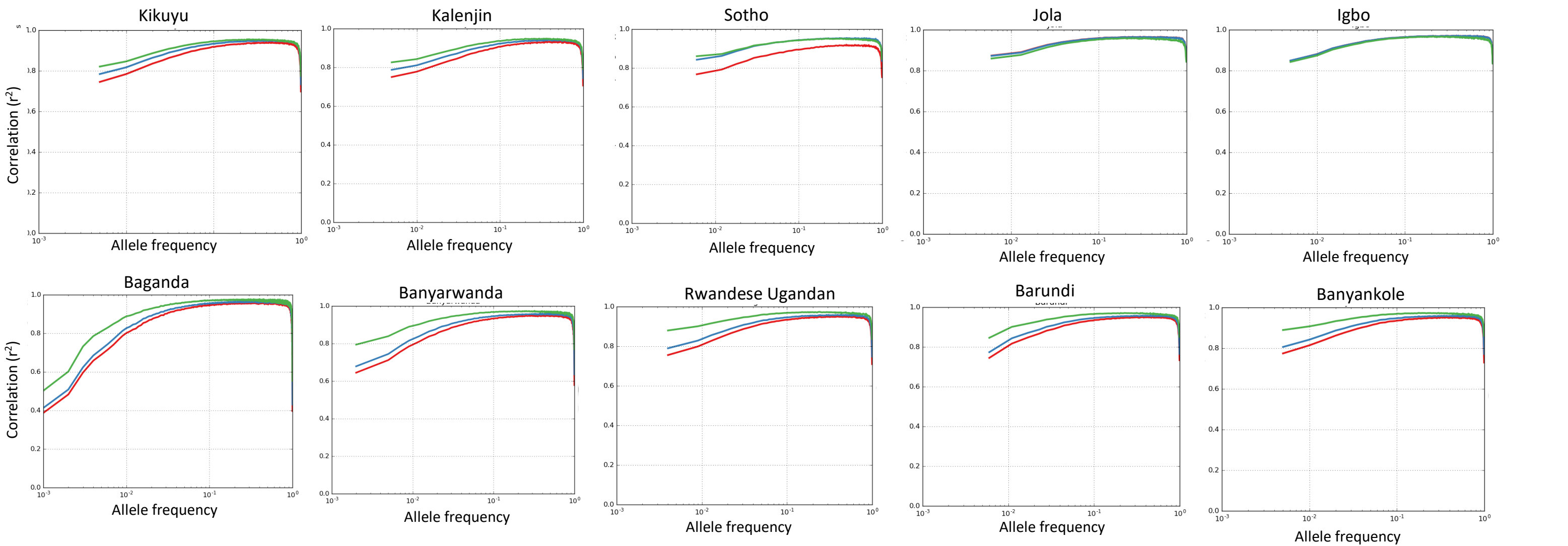
Figure 4: Improvement in imputation accuracy with the UG2G panel
