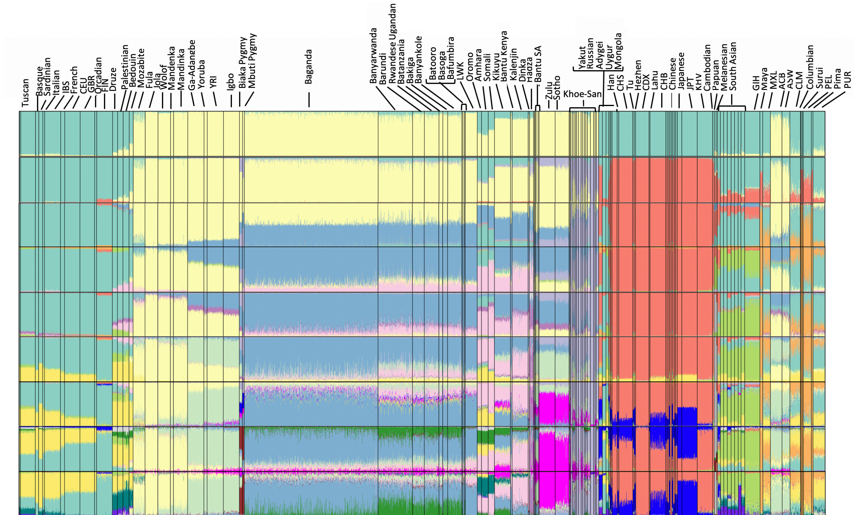
Figure 2: Admixture components in Ugandan population
