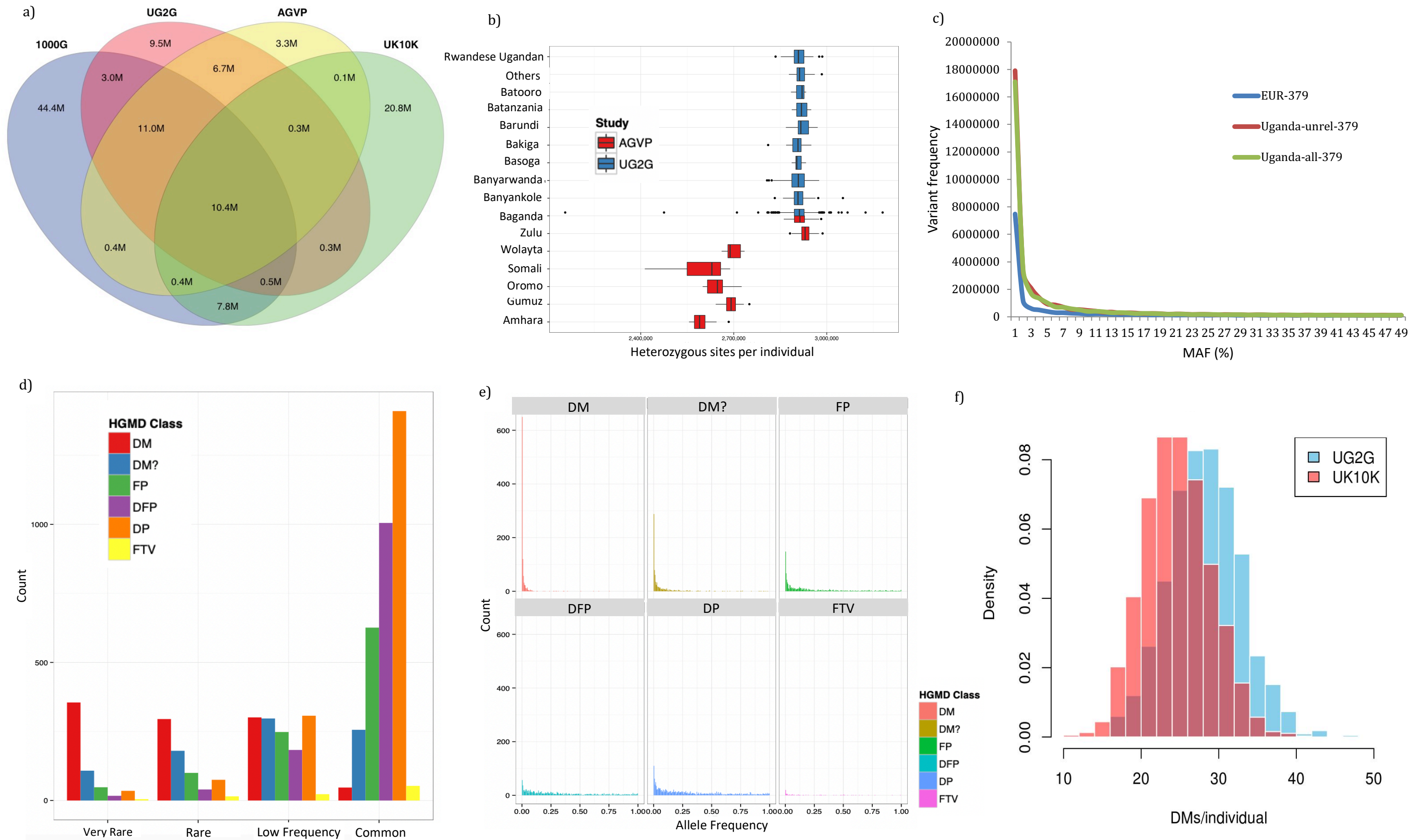
Figure 3. Variant discovery in the UG2G sequence panel
