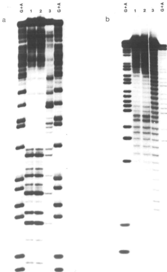
Figure 4. Footprint experiments by DNAase I digestion (a) and by the hydroxyl radical method (b). The procedures are described in Materials and Methods. Lane 1: footprint with NFIII phosphocellulose fraction; lane 2: footprint with crude nuclear extract from Raji cells; lane 3: no protein; G+A: chemical cleavage ladder (32). The weaker bands in the lower part of the gel in Fig. 4b do not represent a second footprint region but are due to lower recoveries of the short cleavage fragments of the 42 bp oligonucleotide after the concentration and precipitation steps. In panel b, the footprint on the complementary strand of oligonucleotide F' is shown.
