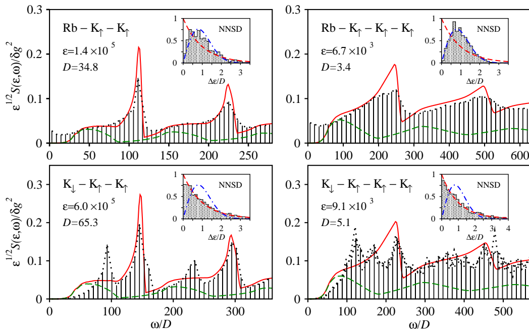
Figure 1: (color online) Dotted lines present dynamic structure factors for nonintegrable (upper panel) and integrable cases (lower panel). Red solid and green dashed lines are the result of the binary approximation (see text). Insets show the nearest neighbor spacing distributions for the ensembles of energy levels used to calculate S in the corresponding parent graphs. Red dashed and blue dash-dotted lines stand, respectively, for the Poissonian and Wigner-Dyson distributions.
