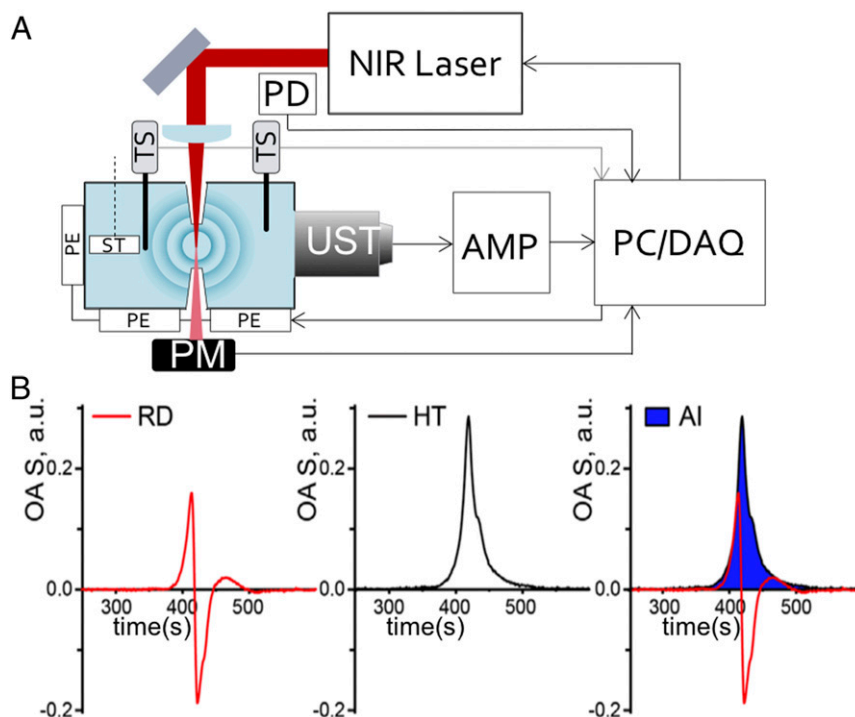
Fig. 1. (A) Schematic representation of the experimental setup for optoacoustic spectroscopy. UST, ultrasound transducer; PD, photodiode; AMP, amplifier; TS, temperature sensor; PM, power meter; ST, stirrer; PE, Peltier element; PC/DAQ, personal computer with data acquisition card. (B) Data processing and analysis steps. OAS raw data (RD, Left ) was transformed by Hilbert transformation (HT, Middle ), and the area of interest (AI, Right in blue) under curves was taken as the intensity of the OAS signal ( I_{OA} ).
