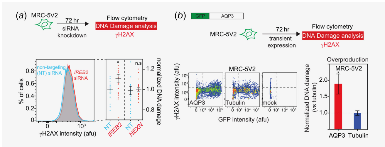
Figure 5. IREB2 knockdown and AQP3 overproduction promote endogenous DNA damage. (a) Knocking down IREB2 , but not NEXN by siRNA causes increased \gamma H2AX level in MRC-5V2 cell line. Upper: scheme for a siRNA DNA damage assay. Lower left: representative flow cytometric histogram showing increased \gamma H2AX in cells with IREB2 knockdown compared to cells that were transfected with nontargeting siRNA. Lower right, a summary of at least three independent experiments for both IREB2 and NEXN , n > 20 . Mean fluorescence intensity of each knockdown experiment was normalized to its corresponding nontargeting siRNA control. Error bar: SEM. (b) AQP3 overproduction increases endogenous \gamma H2AX levels in MRC-5V2. Upper: full-length sequence-verified AQP3 fused with N-terminal GFP fusion (and GFP-Tubulin as a control) were transiently overproduced in MRC-5V2 cell line and the DNA damage levels for both nongreen and green cells were quantified by flow cytometry (details see Methods). Lower left: representative flow cytometric histograms of GFP- AQP3 , GFP-Tubulin, and mock transfection. Lower right: summary, mean \pm SEM, n \geq 8 . [Color figure can be viewed at wileyonlinelibrary.com ]
