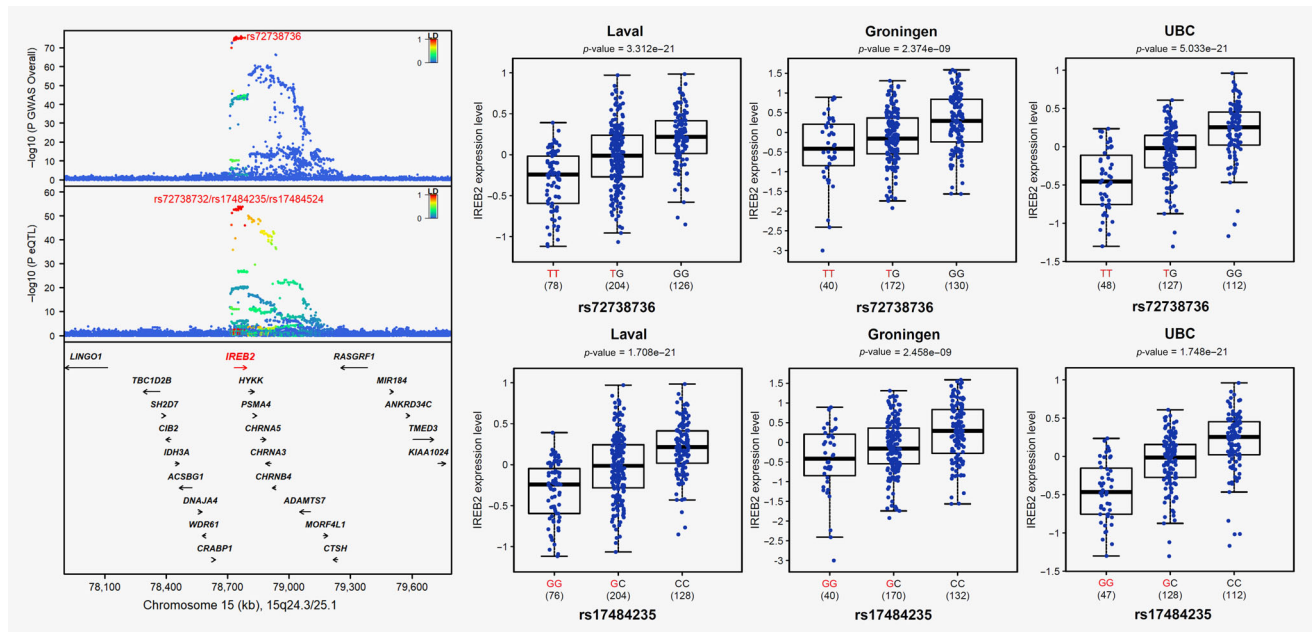
Figure 2. IREB2 is the top candidate target gene on 15q25. The upper left panel shows the genetic associations with overall lung cancer in TRICL-ILCCO OncoArray. The bottom left panel shows the lung eQTL statistics for IREB2 . The location of genes is illustrated at the bottom. The right panel shows boxplots of gene expression levels in the lung according to genotype groups for Laval, Groningen and UBC samples. The y-axis shows the mRNA expression levels. The x-axis shows the three genotype groups for the SNP most strongly associated with lung cancer (upper right) and the SNP most strongly associated with mRNA expression of IREB2 (lower right) with the number of individuals in parenthesis. The risk allele in TRICL-ILCCO OncoArray is shown in red. [Color figure can be viewed at wileyonlinelibrary.com ]
