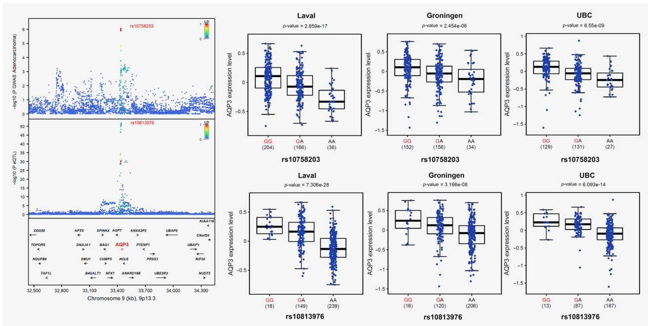
Figure 3. A novel susceptibility locus for adenocarcinoma on 9p13.3 with AQP3 as the underlying gene. The upper left panel shows the genetic associations with adenocarcinoma in TRICL-ILCCO OncoArray. The bottom left panel shows the lung eQTL statistics for AQP3 . The location of genes is illustrated at the bottom. The right panel shows boxplots of gene expression levels in the lung according to genotype groups for Laval, Groningen, and UBC samples. The y-axis shows the mRNA expression levels. The x-axis shows the three genotype groups for the SNP most strongly associated with lung cancer (upper right) and the SNP most strongly associated with mRNA expression of AQP3 (lower right) with the number of individuals in parenthesis. The risk allele in TRICL-ILCCO OncoArray is shown in red. [Color figure can be viewed at wileyonlinelibrary.com ]
