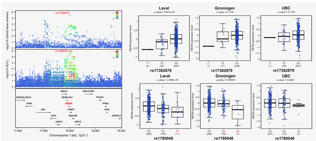
Figure 4. NEXN is the candidate target gene underpinning the lung cancer susceptibility locus for never-smokers on 1p31.1. The upper left panel shows the genetic associations with lung cancer in never-smokers in TRICL-ILCCO OncoArray. The bottom left panel shows the lung eQTL statistics for NEXN . The location of genes is illustrated at the bottom. The right panel shows boxplots of gene expression levels in the lung according to genotype groups for Laval, Groningen, and UBC samples. The y-axis shows the mRNA expression levels. The x-axis shows the three genotype groups for the SNP most strongly associated with lung cancer (upper right) and the SNP most strongly associated with mRNA expression of NEXN (lower right) with the number of individuals in parenthesis. The risk allele in TRICL-ILCCO OncoArray is shown in red. [Color figure can be viewed at wileyonlinelibrary.com ]
