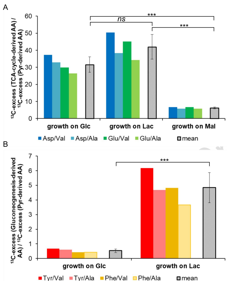
Fig. 5 Marker ratios of ^{13}\text{C} -excess between selected amino acids. (A) ^{13}\text{C} -excess (TCA cycle-derived amino acids) / ^{13}\text{C} -excess (pyruvate-derived amino acids). The coloured bars depict the ratios of the chosen amino acids in three independent labelling experiments with each of the three substrates, glucose (Glc), lactate (Lac) or malate (Mal). The grey bars show the mean values of ^{13}\text{C} -ratios for these fractions. The individual ratios as well as the mean values are significantly higher when an active \text{CO}_2 -fixation is required in the experiments with Glc and Lac compared to a background or random fixation of \text{CO}_2 in the experiment with Mal. p-Values were calculated by Student's t-test (unpaired): p(\text{Glc/Lac}) = 0.05031 , p(\text{Glc/Mal}) = 0.00003 , p(\text{Lac/Mal}) = 0.00006 . (B) ^{13}\text{C} -excess (gluconeogenesis-derived
