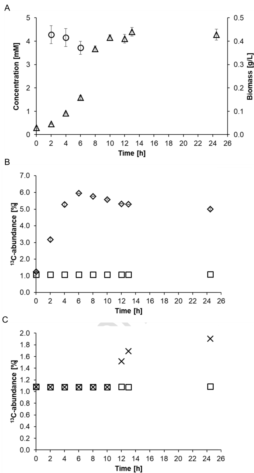
Fig. 2 (A) Glucose consumption and biomass production by B. subtilis W23 growing in M9 medium containing 1 g/ L glucose. The circles represent the glucose concentration and
