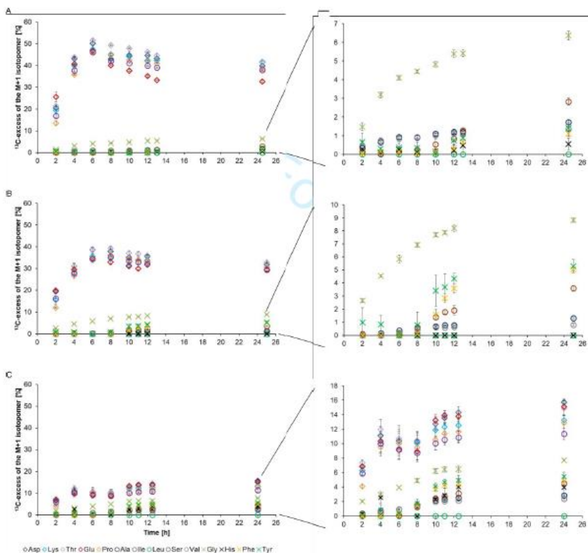
Fig. 4 ^{13}\text{C} -Excess (mol%) of the M+1 isotopomers of specific amino acids produced in \text{H}^{13}\text{CO}_3^- -labelling experiments with glucose (A), lactate (B), and malate (C), respectively. Amino acids depicted as diamonds are derived from the TCA cycle. Amino acids depicted as circles are derived from pyruvate. Amino acids depicted as crosses are derived from the gluconeogenesis pathway. The ^{13}\text{C} -excess of the amino acids derived from pyruvate and the gluconeogenesis pathway are also displayed with a different scaling to improve visibility.
