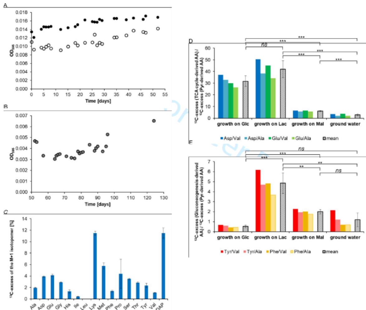
Fig. 7 Labelling experiment with a natural groundwater community and \text{H}^{13}\text{CO}_3^- as a tracer. (A) Growth curves of the bacterial groundwater communities growing on different concentrations of organic fertiliser. The microorganisms that were supplemented with 30 mL of organic fertiliser are depicted as open circles. The microorganisms that were supplemented with 50 mL of organic fertiliser are depicted as full circles. (B) Growth curve of the combined bacterial groundwater community growing on organic fertiliser and soil extract. (C) ^{13}\text{C} -Excess of the M+1 isotopomers of specific amino acids produced by \text{H}^{13}\text{CO}_3^- -labelling experiments. (D) Marker ratios of ^{13}\text{C} -excess between selected amino acids: ^{13}\text{C} -excess (TCA-cycle-derived amino acids) / ^{13}\text{C} -excess (pyruvate-derived amino acids). The coloured bars depict the ratios of the chosen amino acids in the labelling
