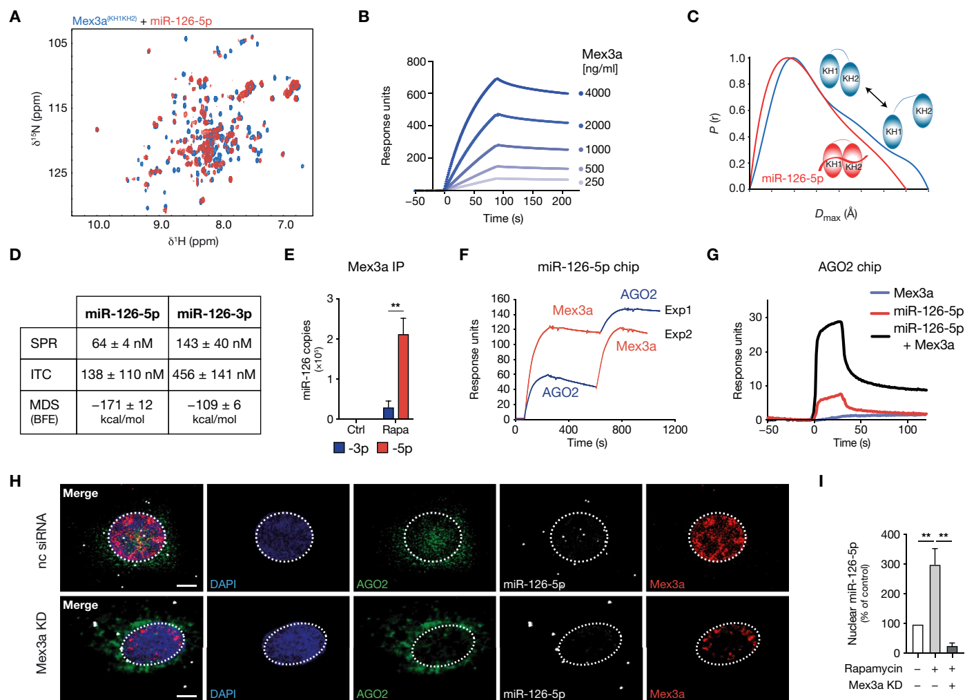
Fig. 4. Mex3a preferentially binds miR-126-5p to drive nuclear enrichment. (A) Overlay of ^1\text{H} - ^{15}\text{N} HSQC spectra of Mex3a (KH1KH2) in the absence (blue cross-peaks) or presence (red) of miR-126-5p (molar ratio, 1:2). (B) SPR sensorgram for interaction between immobilized miR-126-5p and full-length Mex3a. K_D = 3.6 \pm 2.9 nM. (C) Pairwise distance distribution derived from SAXS of Mex3a (KH1KH2) in the absence (blue) or presence (red) of miR-126-5p. (D) Table of estimated binding affinity parameters for the interaction of Mex3a with miR-126-5p and miR-126-3p. (E) RNA-IP of Mex3a in nuclear lysates of HUVECs treated without (Ctrl) and with rapamycin (Rapa) showing miR-126 strand loading ( n = 3 ). (F) SPR sensorgrams showing interaction of sequentially loaded full-length recombinant Mex3a and AGO2 (Exp1) and vice versa (Exp2) on immobilized miR-126-5p. (G) SPR sensorgrams for full-length Mex3a, miR-126-5p, or their combination perfused on AGO2, showing a marked interaction of Mex3a and AGO2 in a complex with miR-126-5p. (H) Representative deconvoluted images for fluorescence in situ hybridization (FISH) for miR-126-5p (gray) and coimmunostaining for AGO2 (green) and Mex3a (red) in rapamycin-treated HUVECs with or without Mex3a KD. Scale bars, 5 \mu\text{m} . (I) Amount of nuclear miR-126-5p in HUVECs upon rapamycin and Mex3a silencing ( n = 5 ). ** P < 0.01 . Two-factor repeated measures ANOVA (E) or univariate ANOVA with Bonferroni post hoc test (I).
