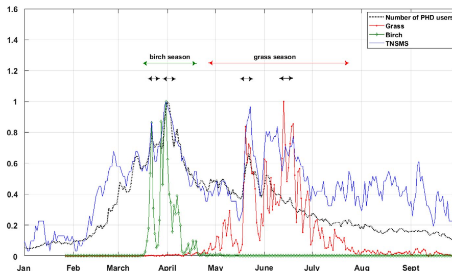
FIGURE 2 Temporal variation of the TNSMS, the number of PHD users, and the birch and grass pollen concentrations for 2014 (mean daily values, Pannonian lowlands region of Austria). The PS per pollen type is marked with arrows with a textual label. The multiple PPP starts-ends are denoted with double arrows. The horizontal axis reports month start. The vertical axis reports the normalized (between zero and one) values of the number of PHD users, the grass, and birch pollen daily concentrations and the TNSMS
