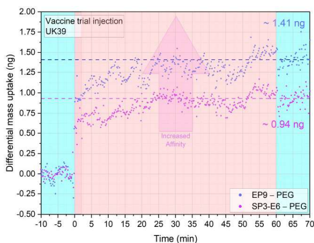
Figure 2 - Antigenic properties of the UK39 antigen as incorporated into the malaria vaccine candidate PEV302. Three sensors were functionalized with EP9 antibodies, three sensors with SP3-E6 antibodies and two with PEG. The PEG functionalised surface works as reference for the differential mass uptake calculation. An injection of 20 \mu l 10 ng/ \mu l at flow
