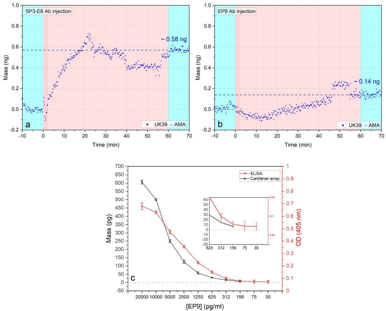
Figure 3 – Antigen binding to the anti-UK39 monoclonal antibodies: SP3-E6 and EP9 (Fig. 3-a,b). Four sensors were functionalized with AMA49-C1 and four sensors with UK39. Two consecutive injections of two different antibodies solutions (SP3-E6 (Left -a) and EP9 (Right - b)) at concentration 0.7 ng/ \mu l and flow rate of 100 \mu l/min were performed (pink portions). Each injection is preceded by a stabilisation time and followed by a wash step in PBS buffer (light blue portions). Differential mass uptake between the two malaria vaccine formulation referring to UK39 and AMA49-C1 was calculated for each different antibody (each data group represents the average of four sensors minus the average of 4 reference sensors with a mass resolution of \pm 15 pg). Direct comparison of dose-response curves of ELISA and cantilever-based bioassay (Fig. 3-c). Response to serial dilutions of individual cantilever-based arrays (black) and ELISA assay (red), both performed with diluted EP9 mAbs were compared. Cantilever-based values were taken at 20 minutes after the injection and their standard deviation obtained by extrapolating the values between 15 and 25 minutes of each experiment. The cantilever specific standard deviation was calculated considering the average of 2 x 4 sensors. The ELISA dilution series was conducted in hybridoma supernatant. Additional details are shown in the supplementary information and in ref 31 . Inset: Zoom to low concentration range.
