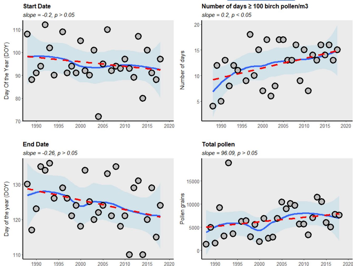
FIGURE 1 Overview on the start and end of birch pollen season, the number of days \geq 100 birch pollen/ \text{m}^3 and the total pollen (annual sum) measured at the pollen station Frauenlobstrasse 9-11 in 80337 Munich, Germany from 1988 till 2018, except of 1995. For every plot, the slope of the fitted regression line indicating a (linear) trend, and the statistical significance of the trend (in terms of P -value) is mentioned. The number of days \geq 100 birch pollen/ \text{m}^3 has a statistically significant trend of increase during the studied period. Dashed red line represents the linear regression line; blue line represents a least squares fit; thick light blue line represents the confidence interval for the aforementioned least squares fit
