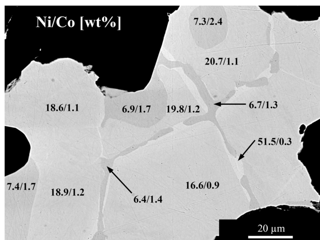
Fig. 8. Details of a metal aggregate within the Renchen breccia. The aggregate includes kamacite ( \sim 7 wt% Ni), taenite ( \sim 20 wt% Ni), and tetrataenite ( \sim 50 wt% Ni). The values “x.x/y.y” represent the Ni and Co-concentrations in wt% as obtained by SEM-EDS.
