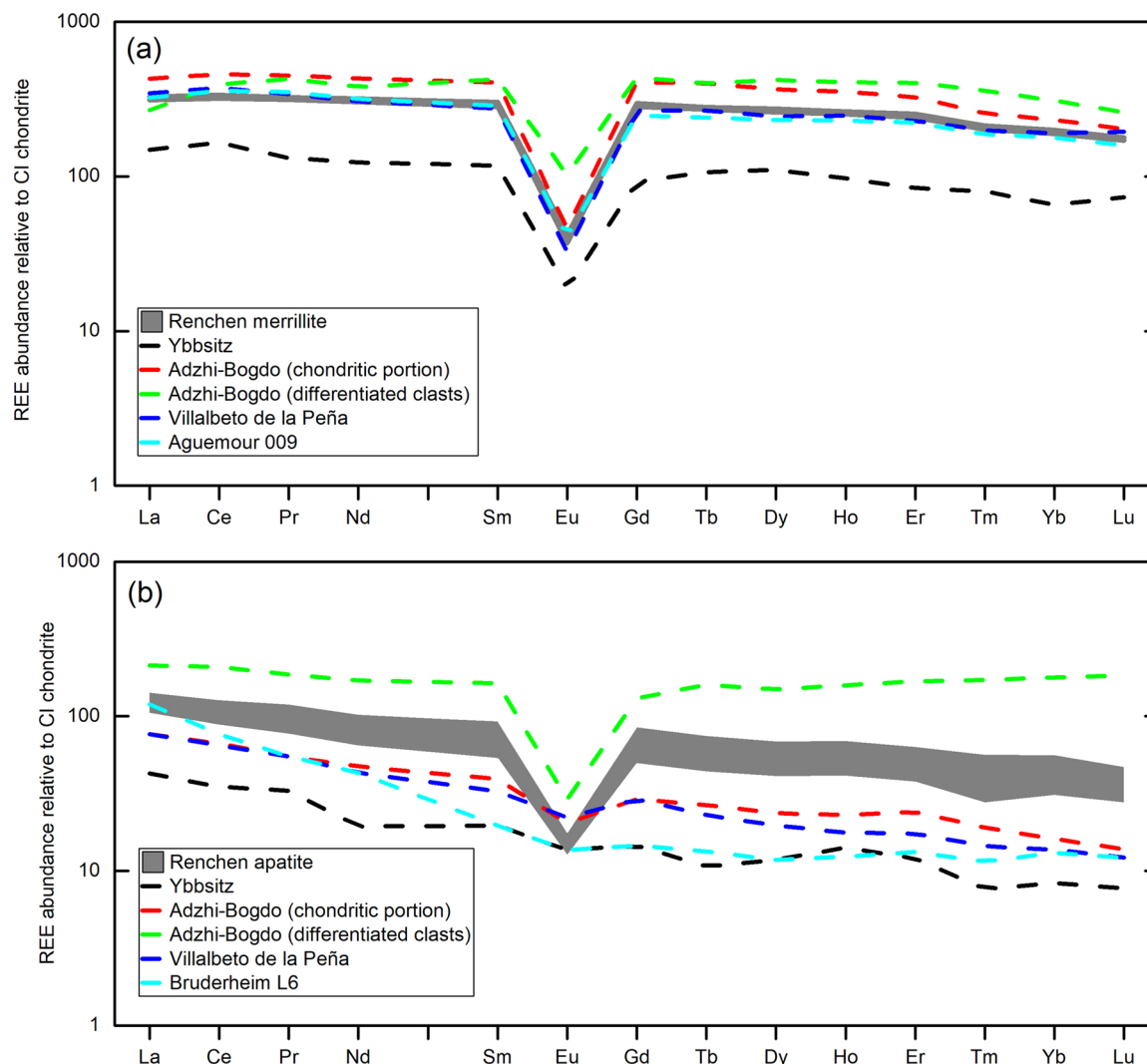
Fig. 7. REE-concentrations of (a) merrillite and (b) apatite from the assemblage shown in Fig. 4a,b normalized to CI (Barrat et al., 2012). The data for the other ordinary chondrites (H4, LL3-6, L6) are taken from Ward et al. (2017).
