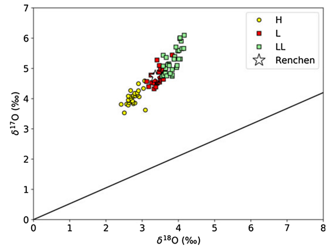
Fig. 12. The O-isotope data for Renchen are consistent with those of other L chondrites. The solid line is the Terrestrial Fractionation Line (TFL).
