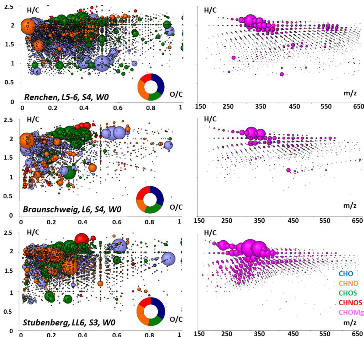
Fig. 14. Van Krevelen diagram visualization in the CHNOSMg space in the negative mode electrospray ionization FTICR-MS illustrates the exact mass data of the methanol soluble organic matter of Renchen, Braunschweig, and Stubenberg meteorites (Bartoschewitz et al., 2017; Bischoff et al., 2017a). The bubble size expresses the relative intensity of the thousands of signals in the experimental mass spectra; the colors in legends represent the components of the left-hand side of the figure (CHO, CHNO, CHOS, CHNOS) and of the right-hand side (CHOMg).
