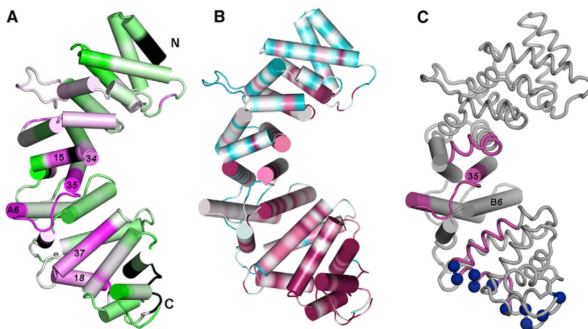
Figure 5. Changes in Hydrogen-Deuterium Exchange at R452 and Amino Acid Sequence Conservation Suggest Sites for G\alpha_i1 Binding
