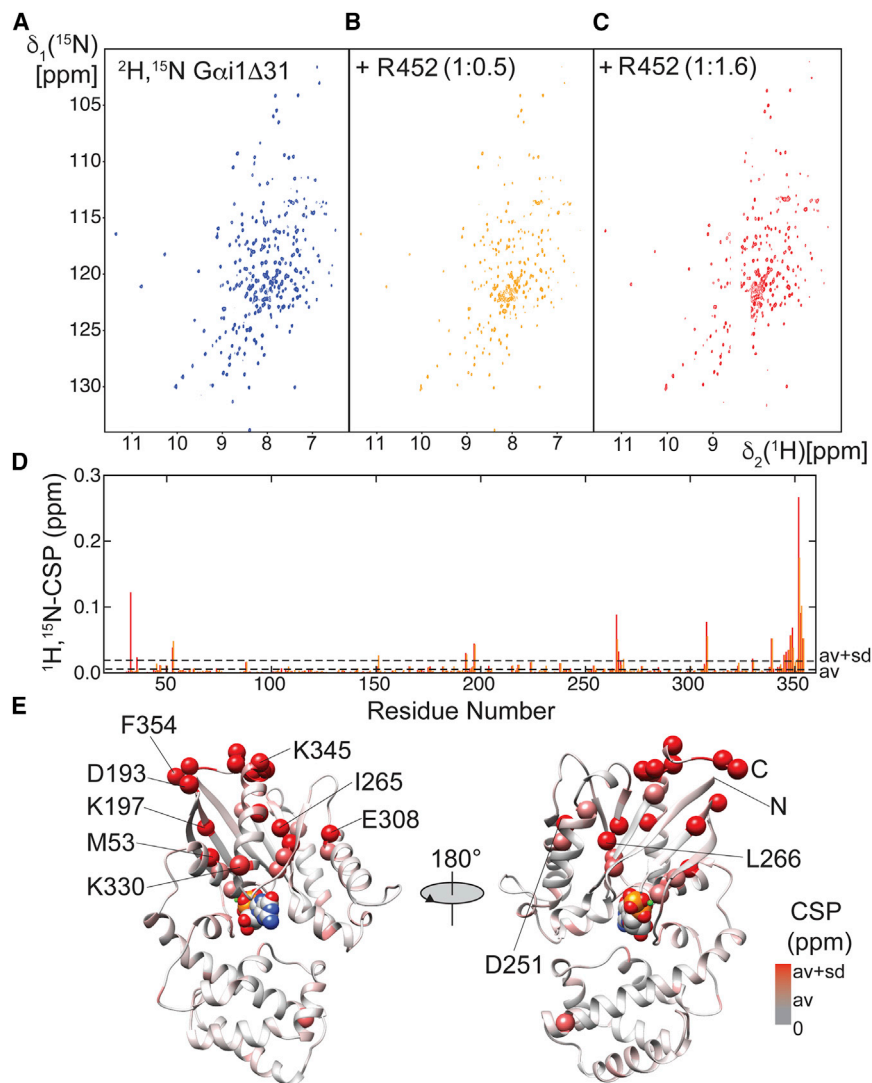
Figure 6. Perturbation of the Structure of Gαi1Δ31 by R452
