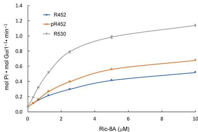
Figure 1. R452 Is an Active Exchange Factor
