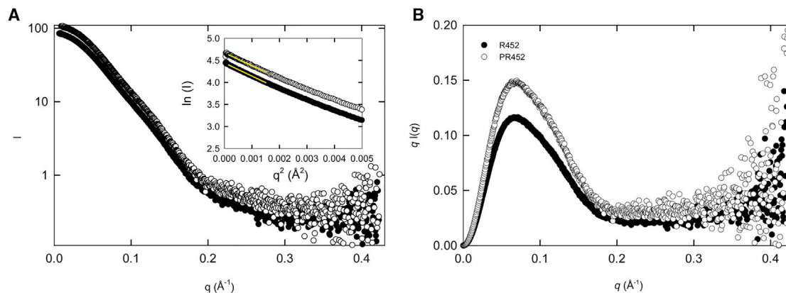
Figure 3. Small-Angle X-Ray Scattering Shows that pR452 and R452 are Well Folded in Solution
